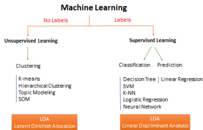
Figure 1 SUPERVISED LEARNING & UNSUPERVISED LEARNING
