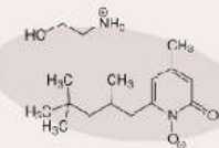
Piroctone Olamine
