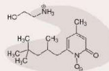
Piroctone Olamine
