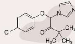
Climbazole
