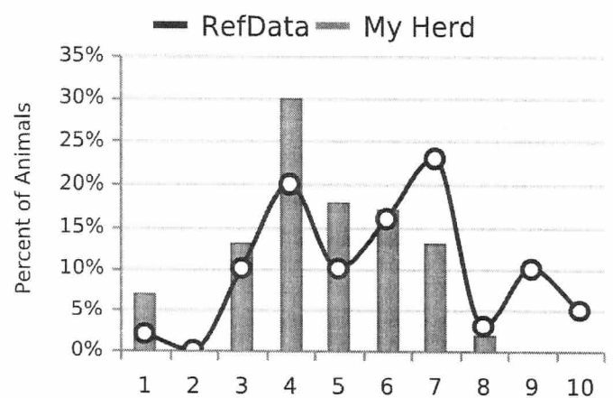
Tndr Score
