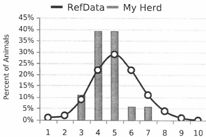
RFI-Taurus Score
