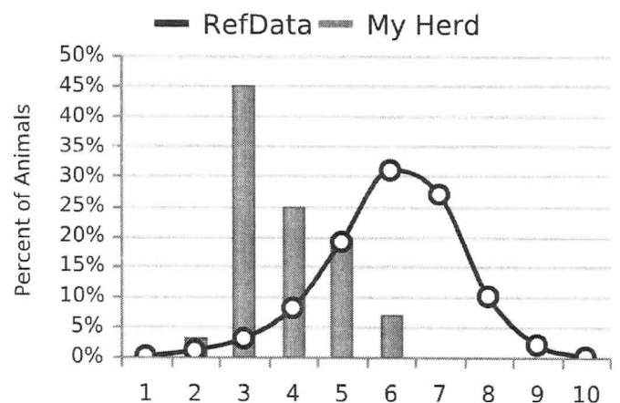
Tndr Score
