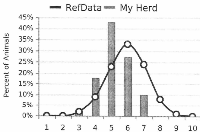
RFI-Taurus Score
