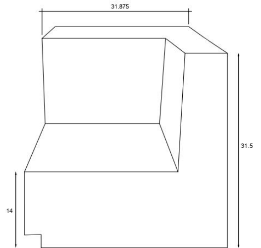
End Section
