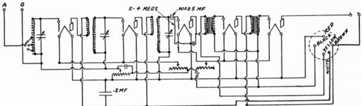
FIG. 46. SCHEMATIC DIAGRAM OF MODEL 10B.
