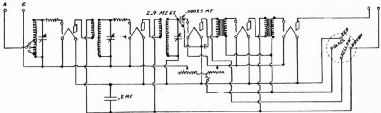
FIG. 44. SCHEMATIC DIAGRAM OF MODEL 10.
