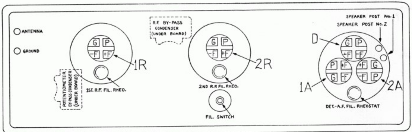
FIG. 45. TOP CHART OF MODEL 10B.
