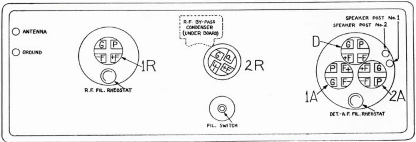
FIG. 43. TOP CHART OF MODEL 10.
