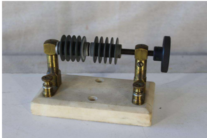
148: Early Spark Gap
