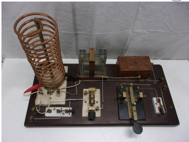
142: Spark Transmitter
