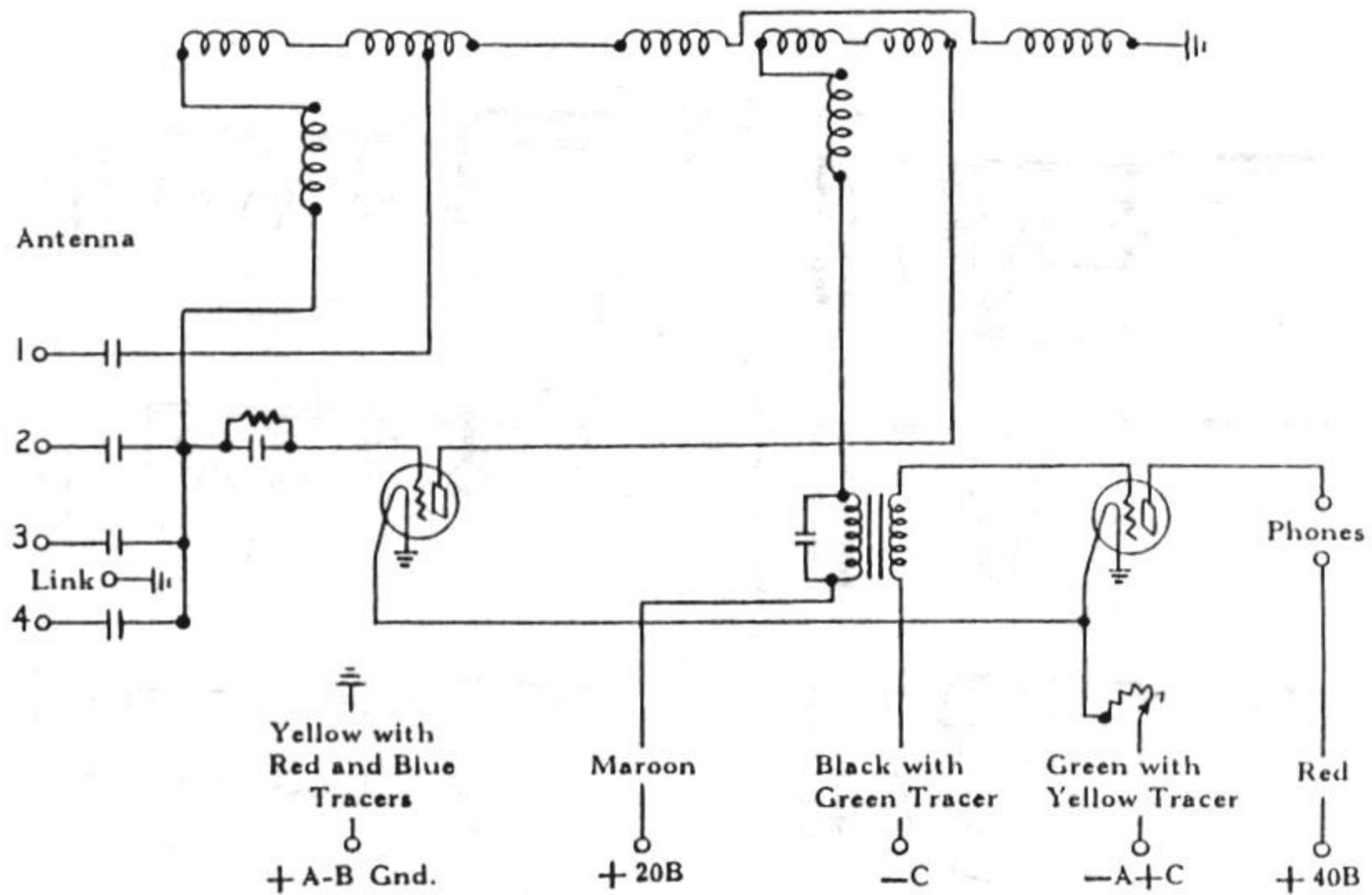
Fig. 4—Diagram of Connections
