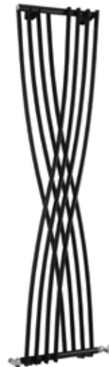
F03827 Contour designer radiator. W450 H1775. Output 2436 Btu/hr. Pipe centres 450mm. Anthracite
