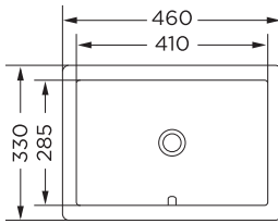
F02600 Square basin W460 H190 D330
