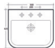
F04458 Series 600 500mm inset basin 1TH W500 H190 D425
