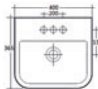
F04442 Series 600 400mm 1TH W400 H180 D365
