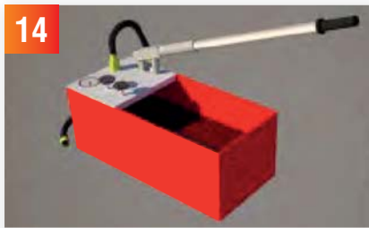
Upon completion of the underfloor heating pipe circuits - ensure all pipe work is pressured tested ( conforming to BS EN 1264).
