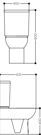
Pavia Close Coupled Toilet
