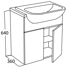
Height with legs - 820mm Basin sold separately
