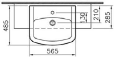
Rosetta Semi-Recessed Basin
