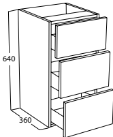
Height with legs - 820mm
