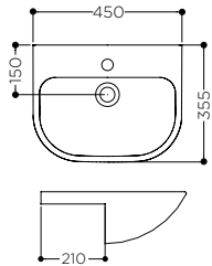
Pavia Semi-Recessed Slimline Basin
