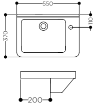
Forino Semi Recessed Slimline Basin
