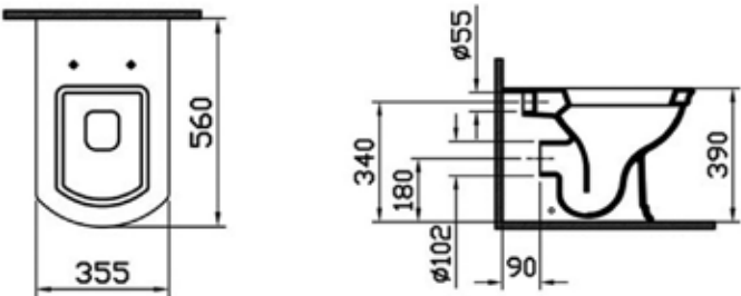
Rosetta Back To Wall Toilet
