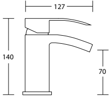
Basin Mixer 0.1 BAR Includes clicker waste BL/PEAKBM £211
