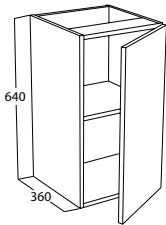
Height with legs - 820mm
