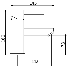
Basin Mixer 0.2 BAR Includes clicker waste QUADBМ £97
