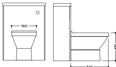
FORINO Comfort Height Toilet. M/FORCHWC/SC. £308
