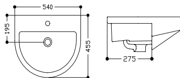
FARO Semi-Recessed Basin. M/FAROCTW. £135
