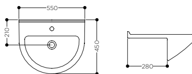
FORINO Semi Recessed Basin. M/FORCTW. £185
