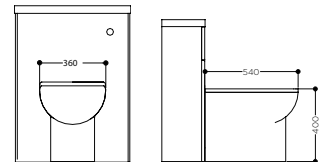
PAVIA Back To Wall Toilet. M/PAVW/WC/S. £300
