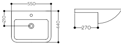
PAVIA Semi-Recessed Basin. M/PAVCTW. £152
