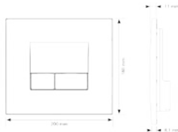
FLUSH PLATE and compatible CISTERN
