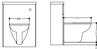
PAVIA Suspended Toilet. M/PAVSW/WC/S. £325
