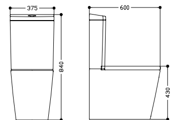
FARO Close Coupled Toilet. M/FAROCCWC/S. £451
