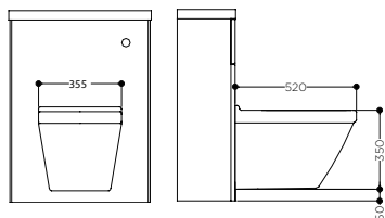
FORINO Suspended Toilet. M/FORSWC/S. £399
