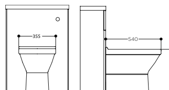
FORINO Back To Wall Toilet. M/FORWC/S. £401
