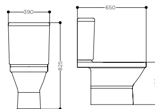
FORINO Close Coupled Toilet. M/FORCCWC/S. £595
