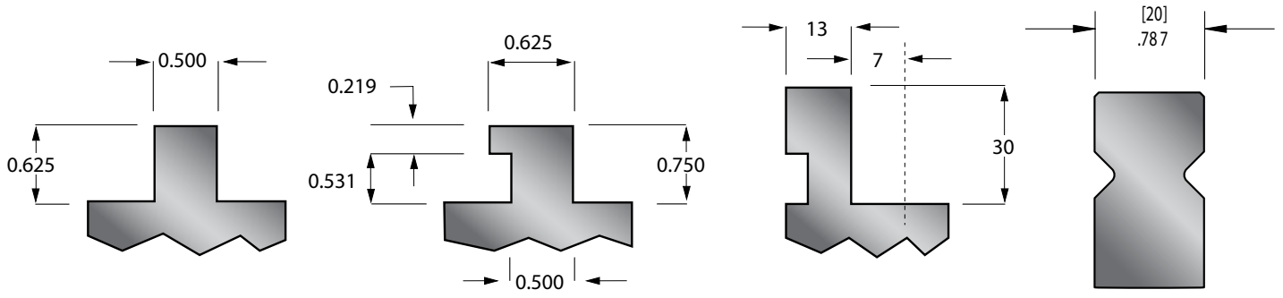
CONVENTIONAL STANDARD (NO SAFETY HOOK)
