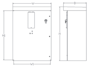
Floor-mount (CX3R-8)
