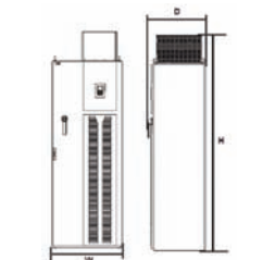
Floor-mount (PX12-8)
