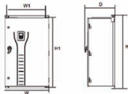
Floor-mount (PX1-8)
