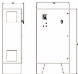
Wall-mount (CX12-10)
