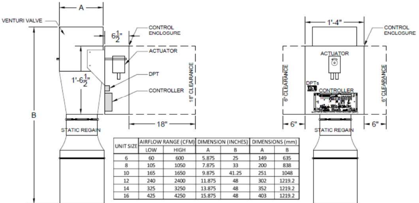
VALVE WITH LARGE ENCLOSURE
