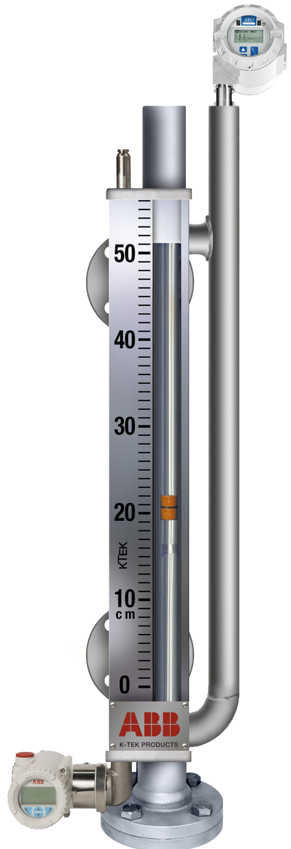
MagWave® Dual Chamber Magnetic Level Gauge
