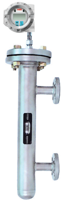
EC External chamber
