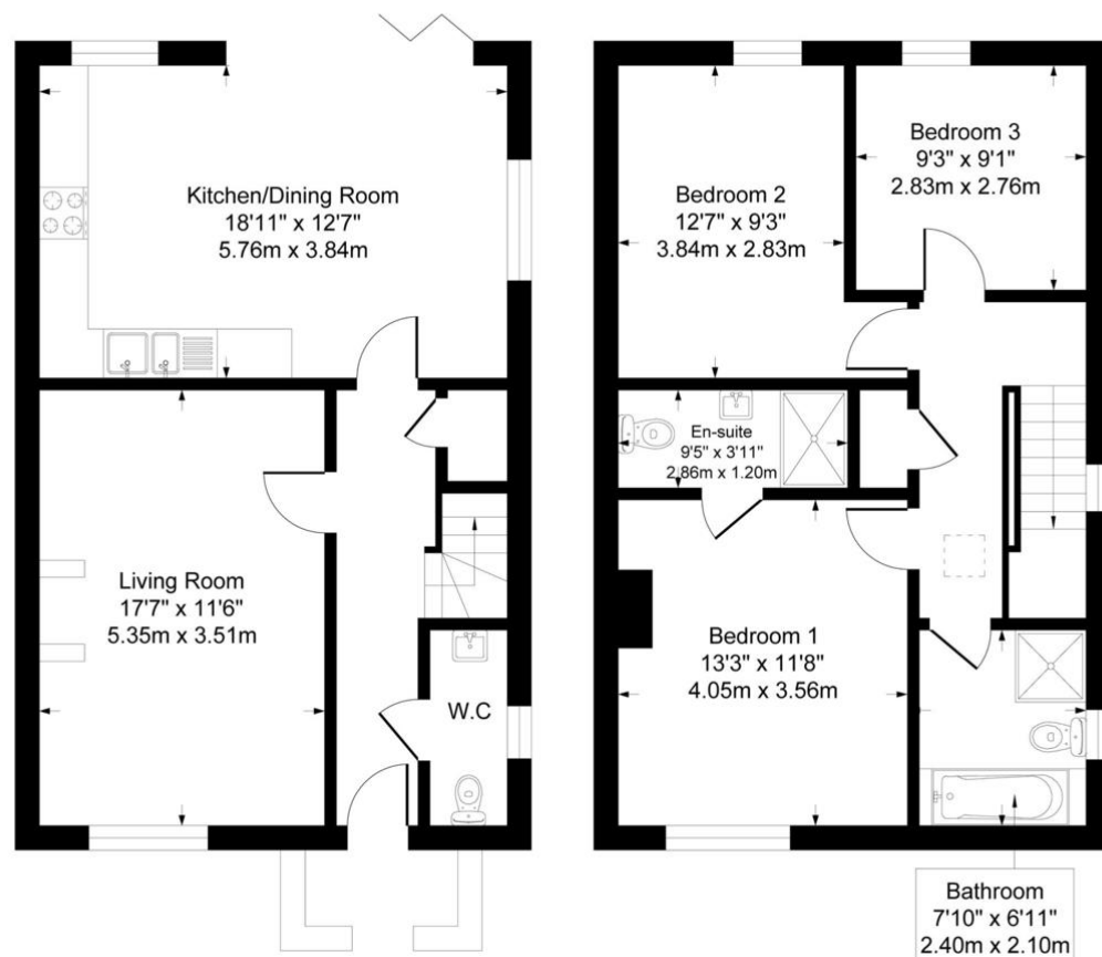
Ground Floor
