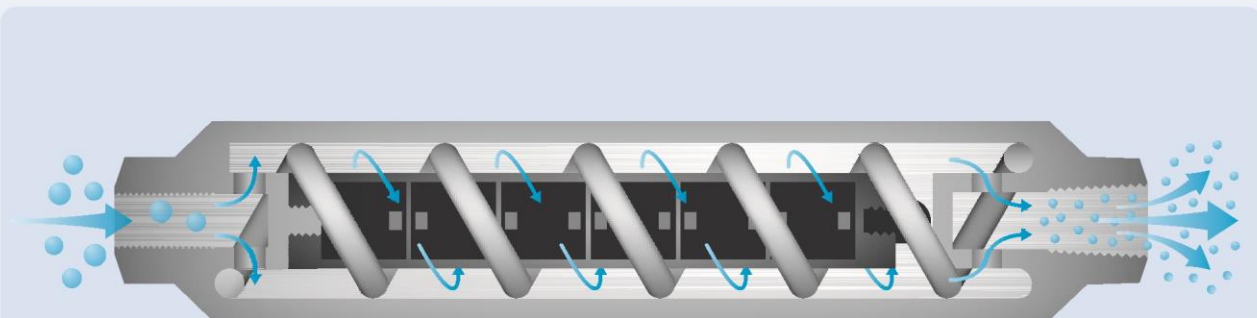
Cross Section of WaterHealer™
