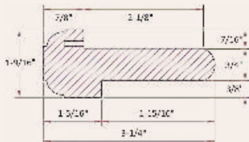
MTAST3480 3/4" Mahogany T-Astragal 8-0 96" (1-3/4" thick door) KASTAST3480 3/4" Knotty Alder T-Astragal 8-0 96" (1-3/4" thick door)
