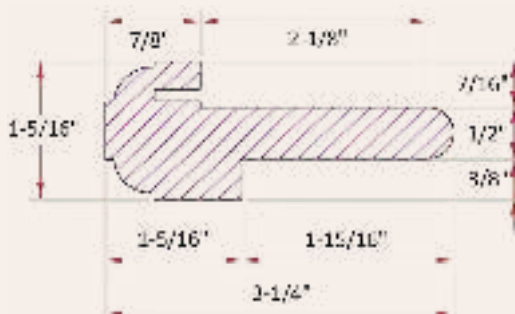
MTAST1280 1/2" Mahogany T-Astragal 8-0 96" (1-3/4" thick door) KASTAST1280 1/2" Knotty Alder T-Astragal 8-0 96" (1-3/4" thick door)
