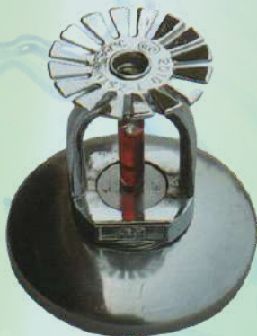
WB 016 1/2" ₱178 WB 016 3/4" ₱250 PENDENT TYPE FIRE SPRINKLER (FOR WALL)
