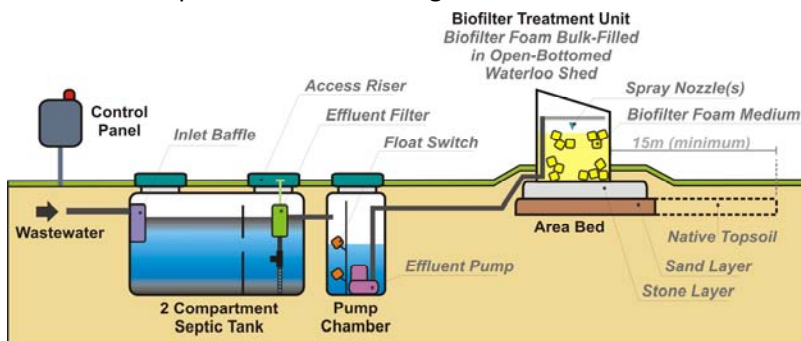
Schematic overview of the Waterloo Shed Biofilter configuration
