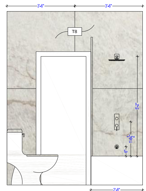
3 WALL ELEVATION
