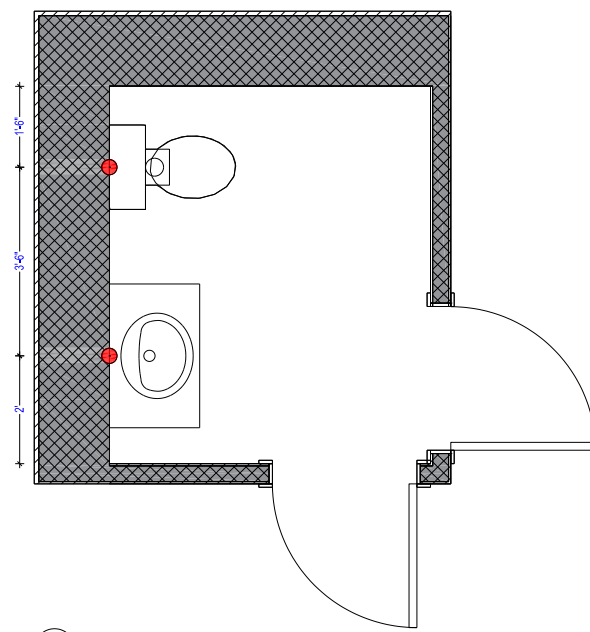
A-16 BATHROOM PLUMBING PLAN
