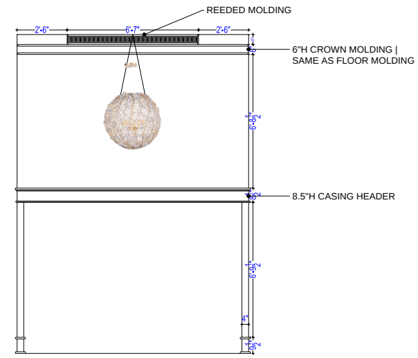
4 DINING ROOM DOORWAY ELEVATION
