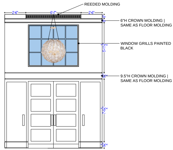
2 FRONT DOOR ELEVATION
