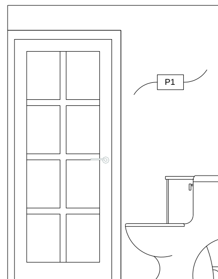
3 WALL ELEVATION
