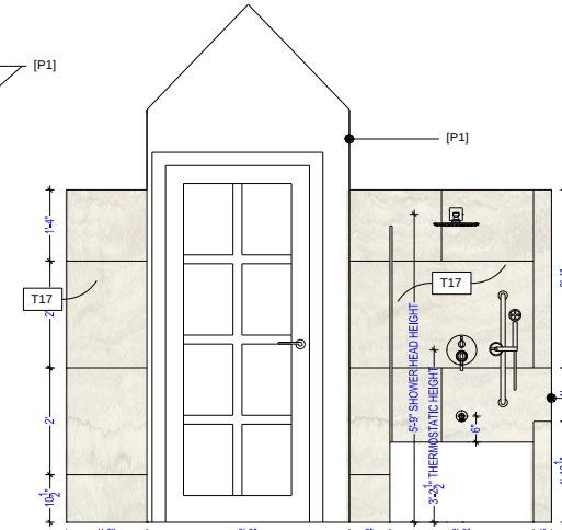
4 WALL ELEVATION
