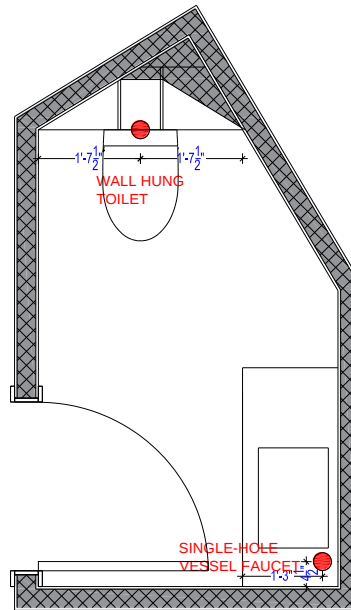
A-8 BATHROOM PLUMBING PLAN
