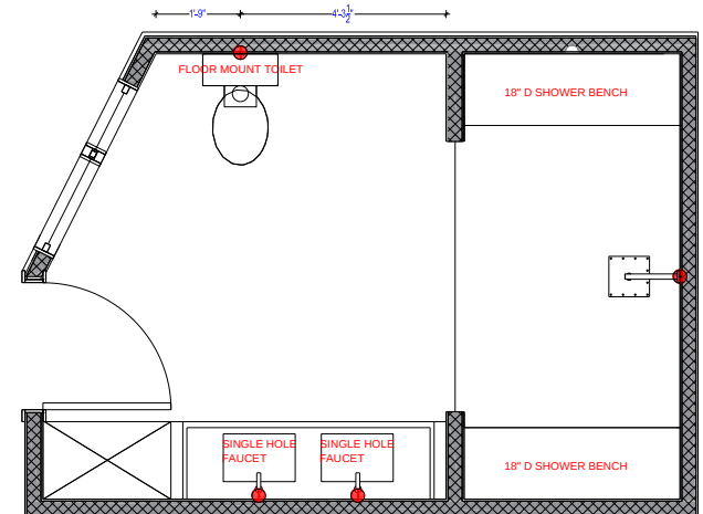
(A-9) BATHROOM PLUMBING PLAN
