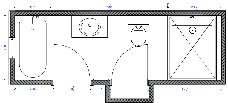
A-10 FLOOR PLAN W/ DIMENSIONS
