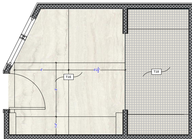
(A-9) FLOOR TILE PLAN
