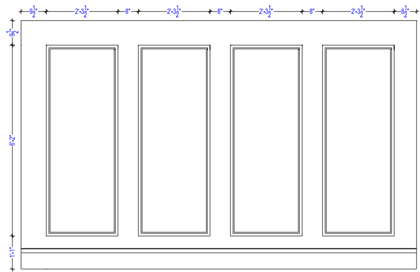
1 HALLWAY ELEVATION
