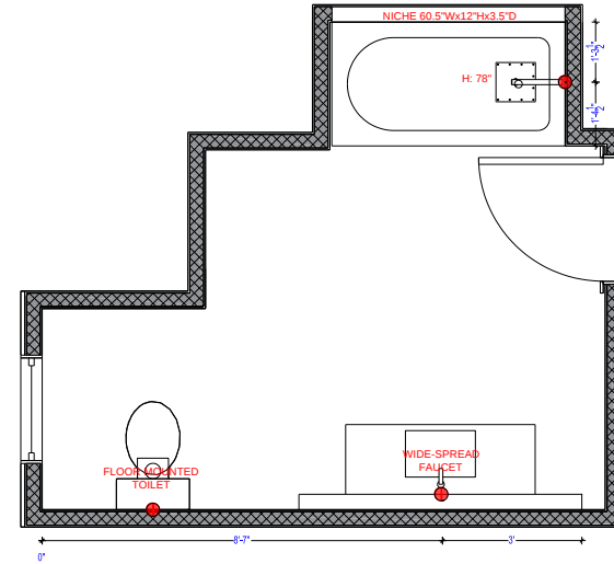
A-14 BATHROOM PLUMBING PLAN
