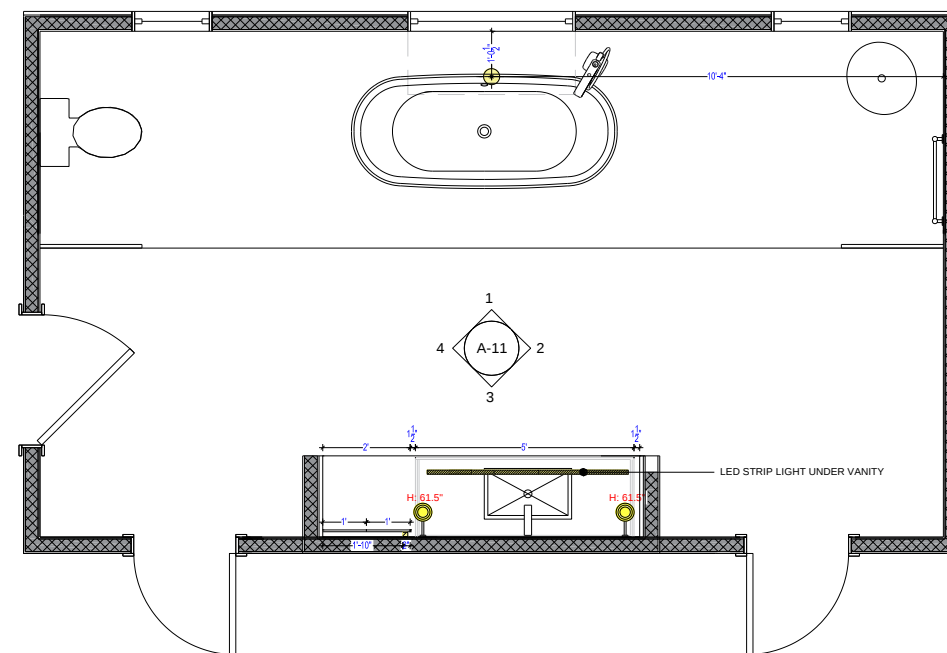
(A-11) LIGHTING PLAN
