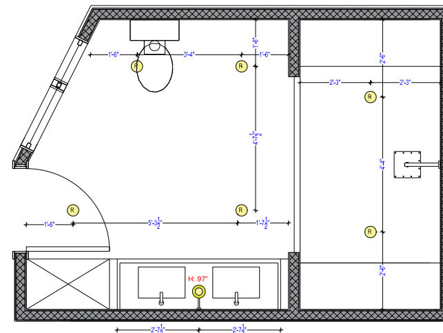
(A-9) LIGHTING PLAN
