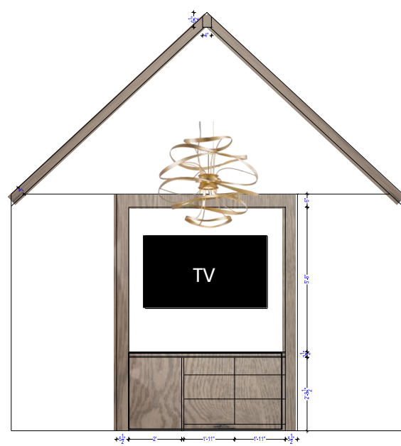
3 WALL ELEVATION
