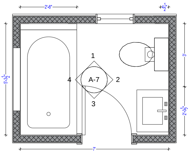
A-7 FLOOR PLAN W/ DIMENSIONS
