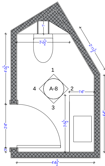
A-8 FLOOR PLAN W/ DIMENSIONS
