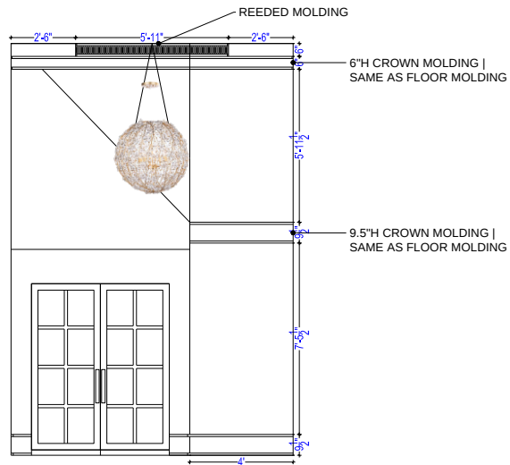
1 POOL ROOM HALLWAY ELEVATION
