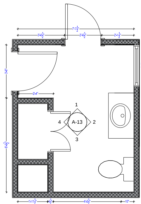
A-13 FLOOR PLAN W/ DIMENSIONS
