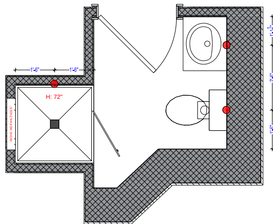
A-17 BATHROOM PLUMBING PLAN
