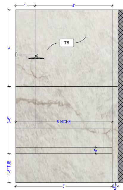
4 WALL ELEVATION
