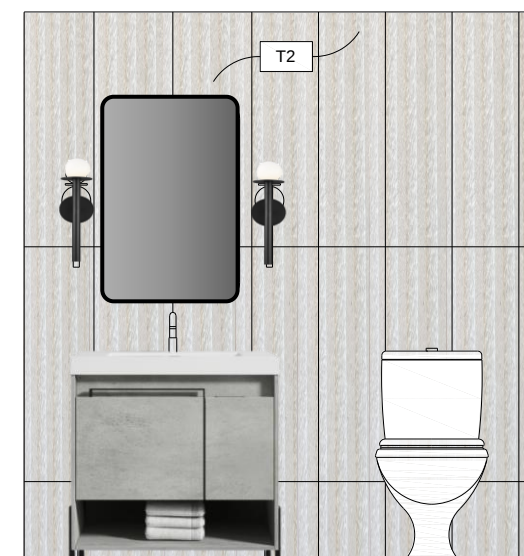
4 WALL ELEVATION
