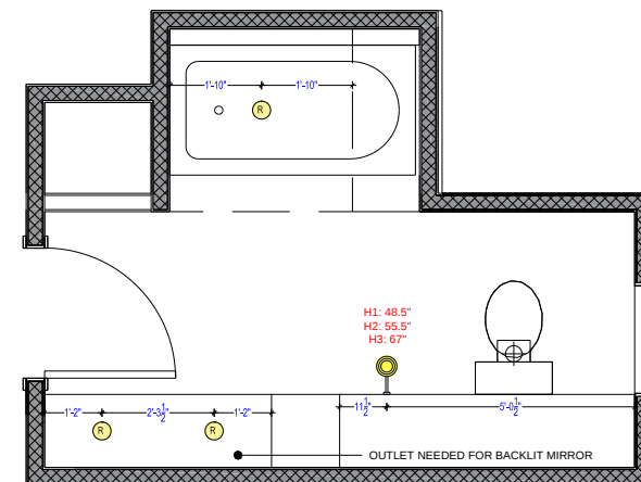
A-15 LIGHTING PLAN
