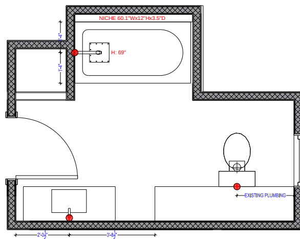
A-15 BATHROOM PLUMBING PLAN
