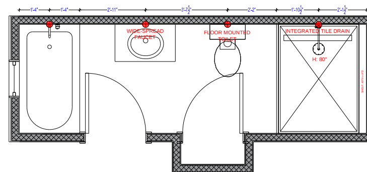
A-10 BATHROOM PLUMBING PLAN
