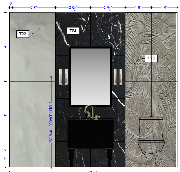
2 WALL ELEVATION
