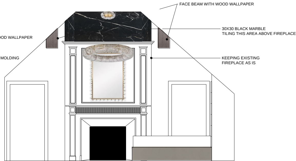
2 WALL ELEVATION
