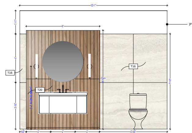
3 WALL ELEVATION
