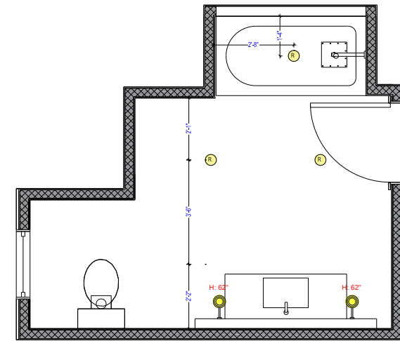
A-14 LIGHTING PLAN
