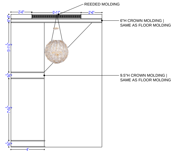
3 LEFT HALLWAY ELEVATION
