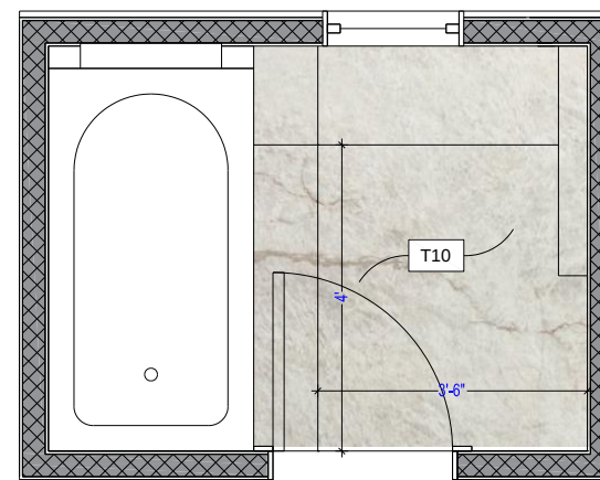
A-7 FLOOR TILE PLAN
