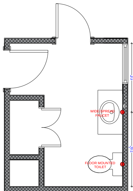
A-13 BATHROOM PLUMBING PLAN
