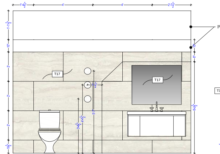
3 WALL ELEVATION
