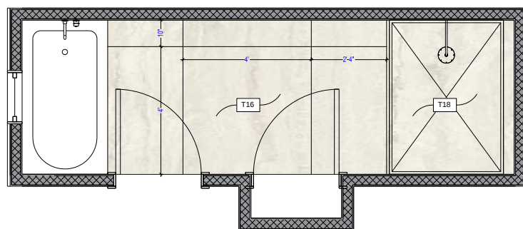
A-10 FLOOR TILE PLAN
