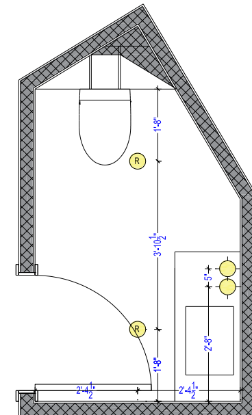
A-8 LIGHTING PLAN
