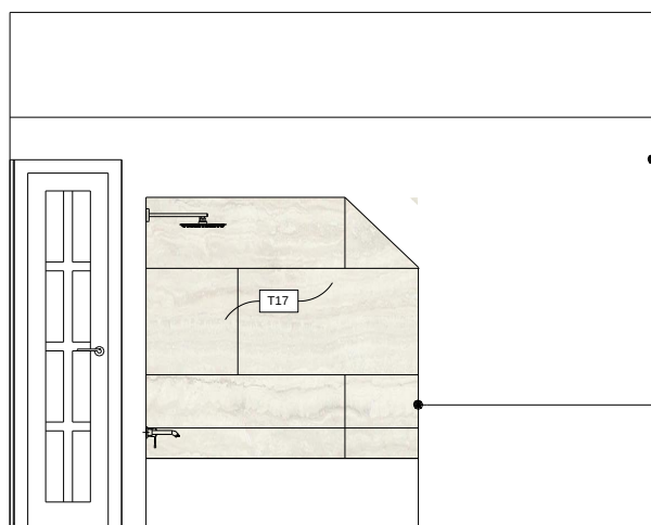
1 WALL ELEVATION
