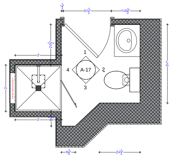
A-17 FLOOR PLAN W/ DIMENSIONS
