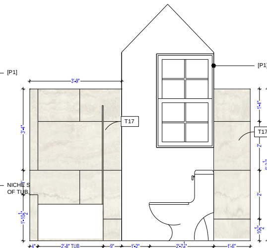
2 WALL ELEVATION
