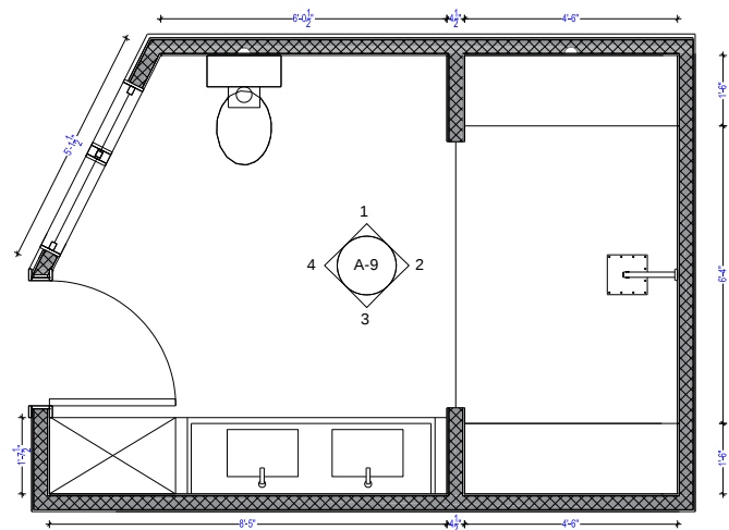
(A-9) FLOOR PLAN W/ DIMENSIONS
