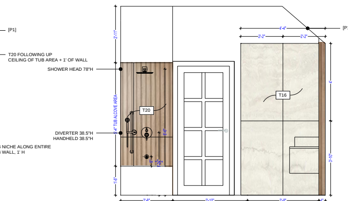
2 WALL ELEVATION
