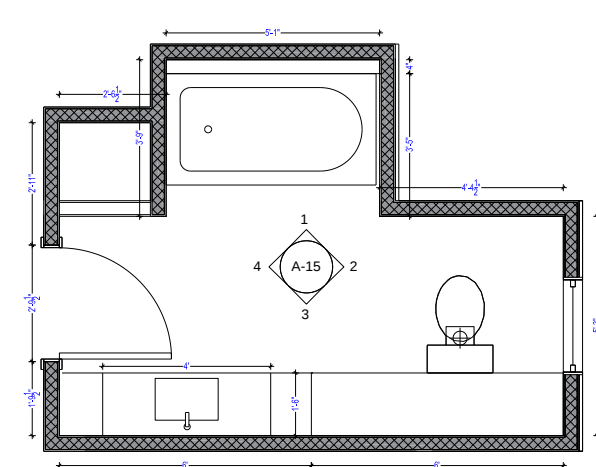
A-15 FLOOR PLAN W/ DIMENSIONS
