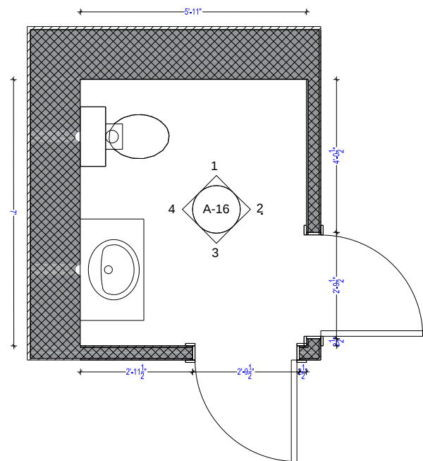
A-16 FLOOR PLAN WITH DIMENSIONS
