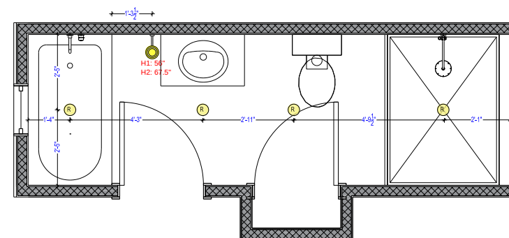
A-10 LIGHTING PLAN
