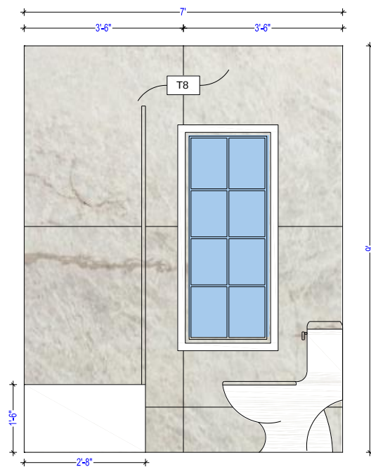
1 WALL ELEVATION
