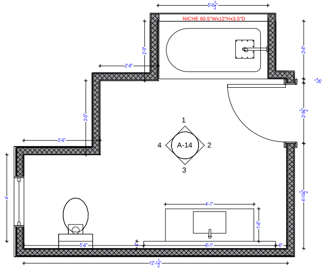
A-14 FLOOR PLAN W/ DIMENSIONS
