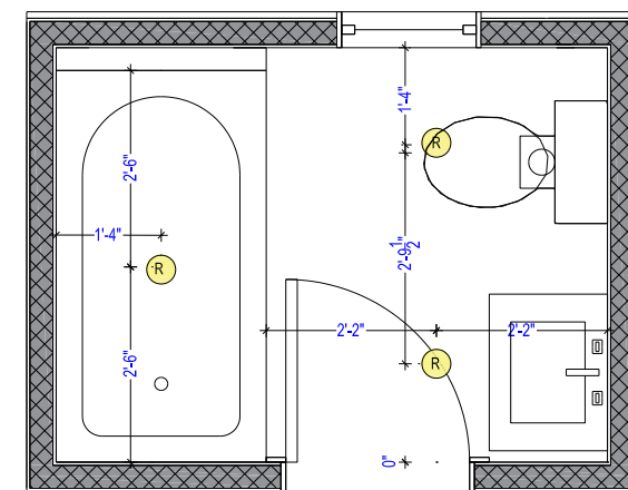
A-7 LIGHTING PLAN
