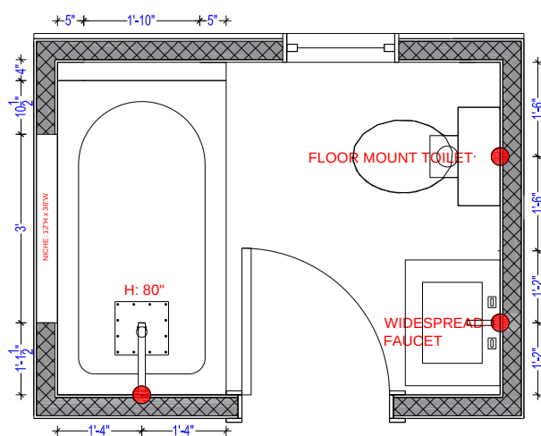
A-7 BATHROOM PLUMBING PLAN
