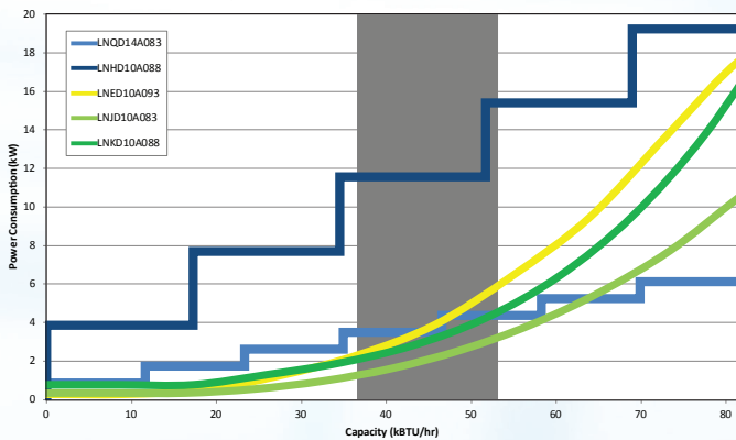
Power Consumption & Variable Speed Operation
