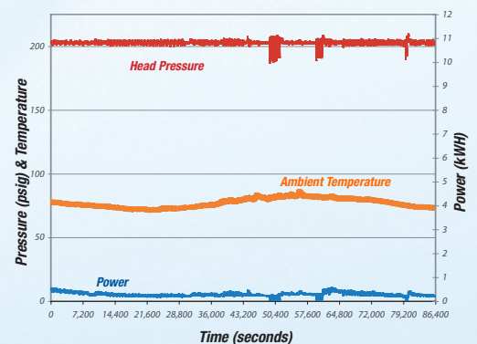
Larkin VSEC Motors Performance
