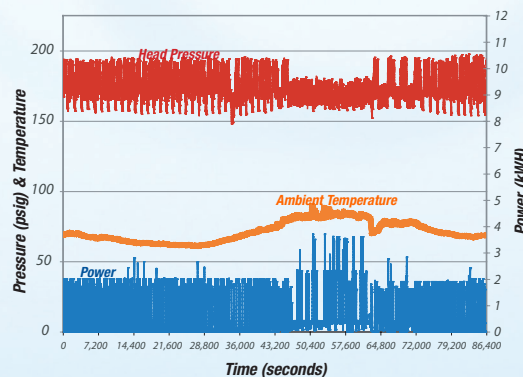
Standard Larkin 1140 RPM Performance
