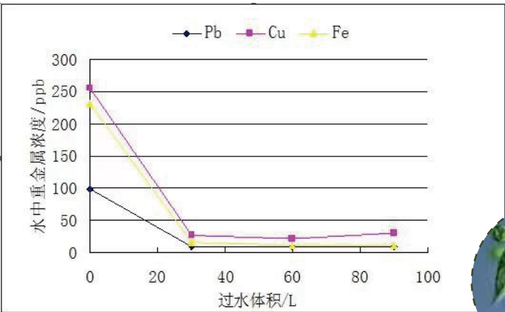
KDF去除金属效果 KDF metal removal effect
