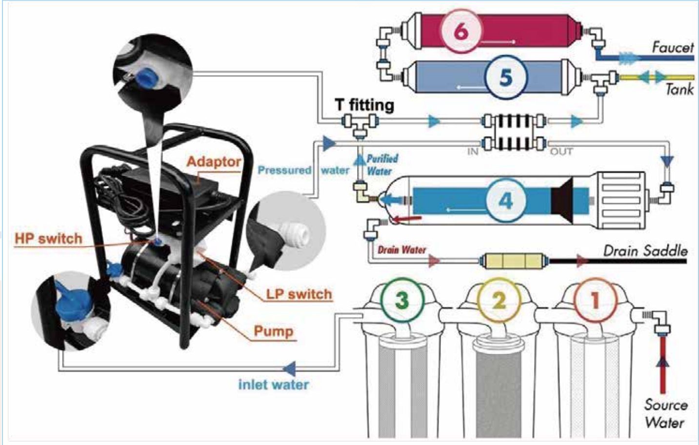
场景1：RO前置增压泵 Scenario 1: RO front booster pump
