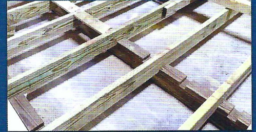
12" On-Center Floor Joists 16" OC is Standard
