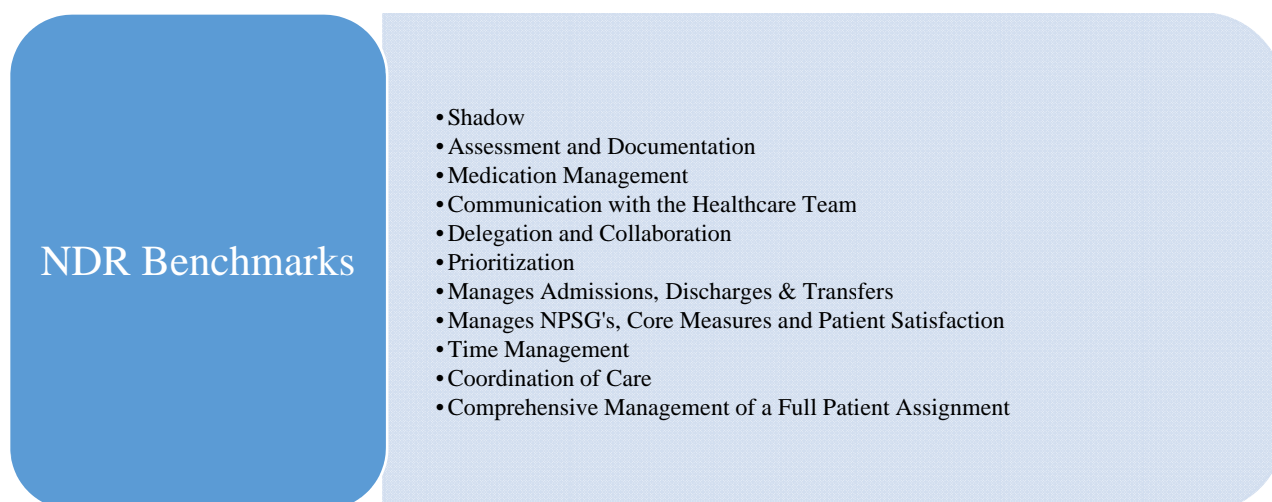
Fig. 2 Benchmark categories.
