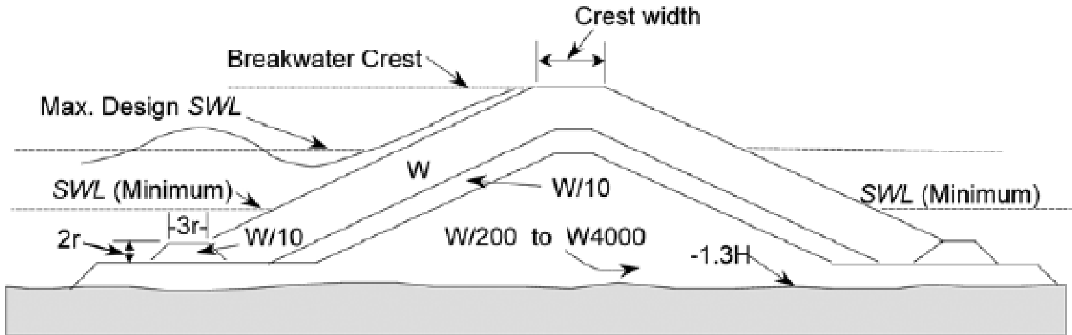
Recommended Three-layer Section
