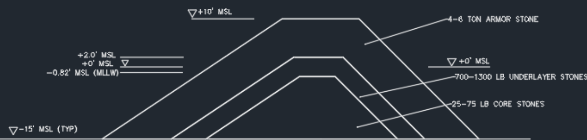
Modified Cross-Section
