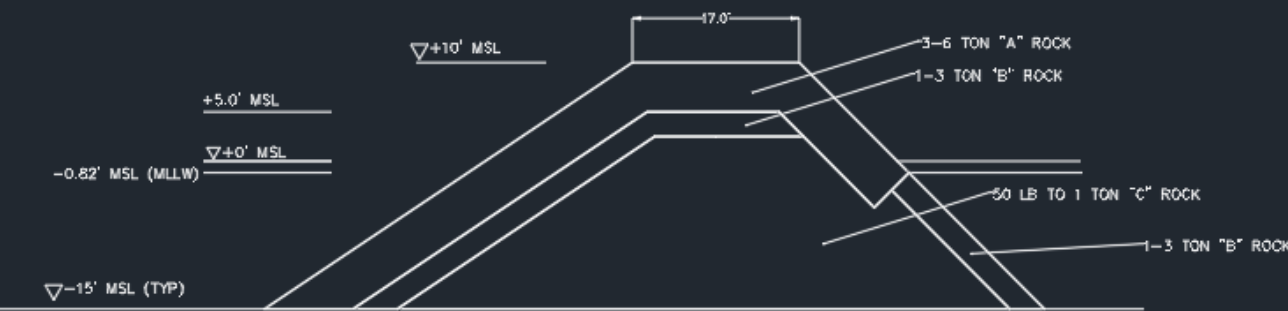
As-Built Cross-Section
