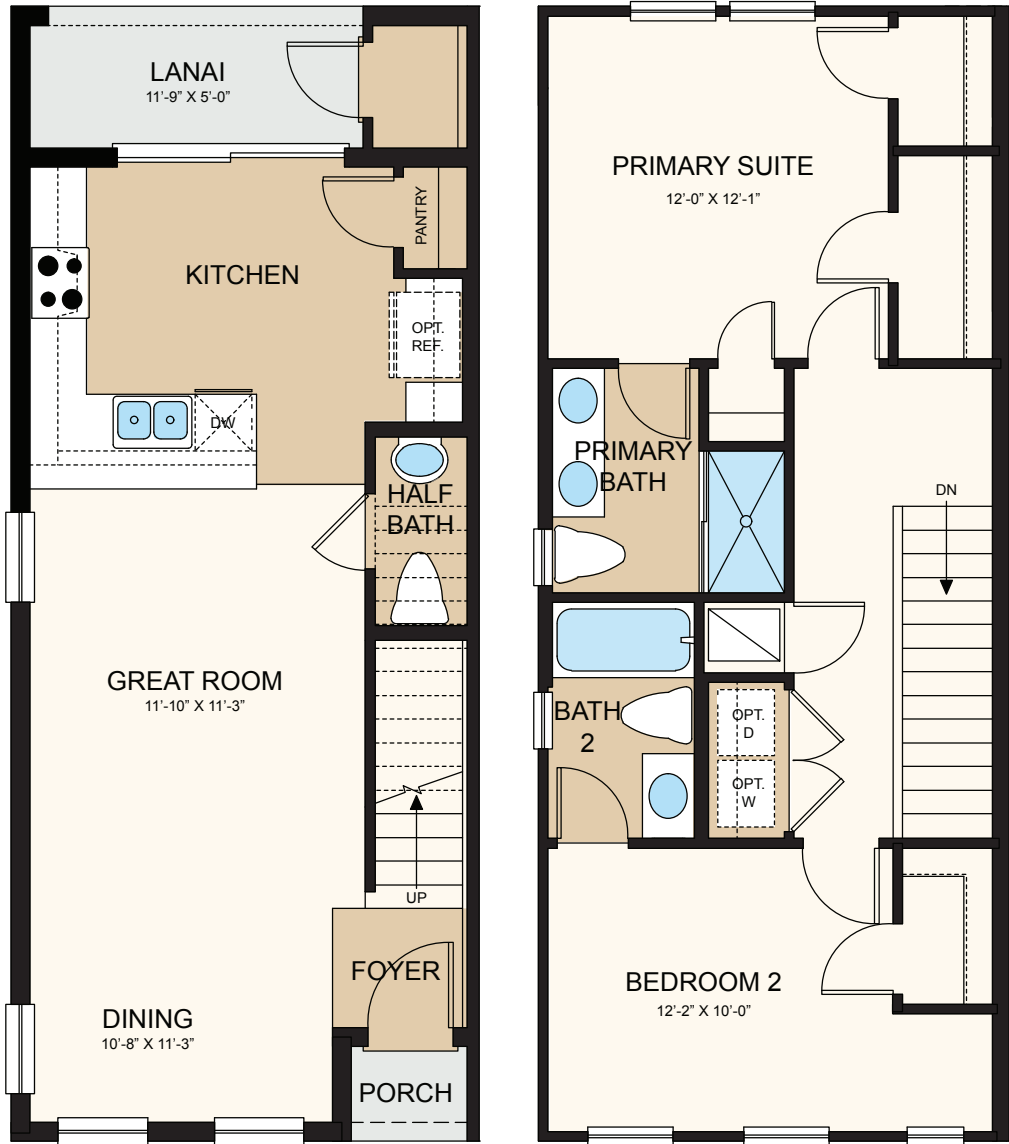
FIRST FLOOR
