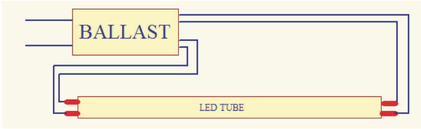
b. One electronic ballast two LED tube
