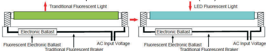
C: Replace electronic ballast Tube (OK)
