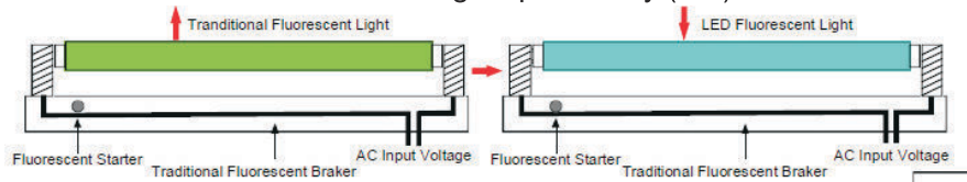
B: Replace Inductive ballast Tube (NO)
