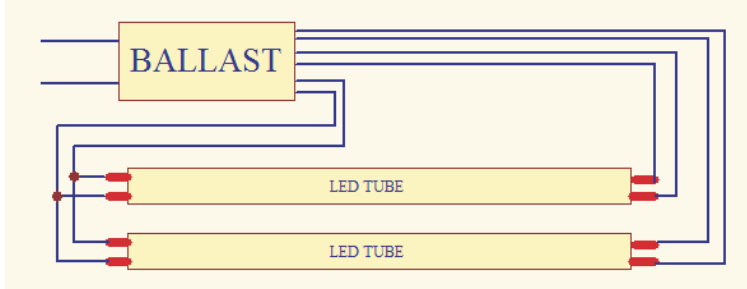
C. One electronic ballast three LED tube
