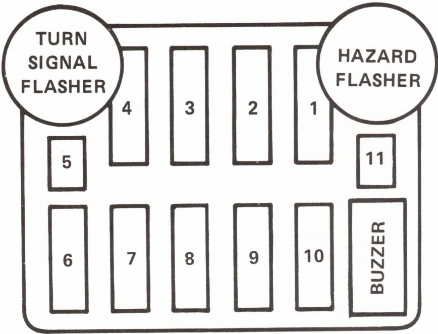
Figure 1 – Fuse Block
