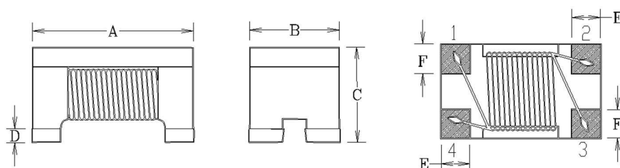
Dimensions (mm)
