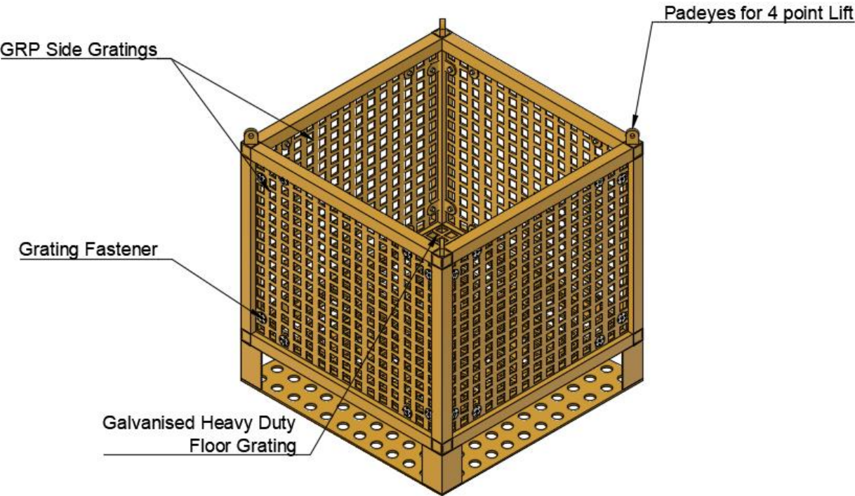
NE Isometric View
