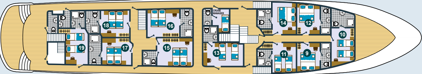
MAIN DECK
