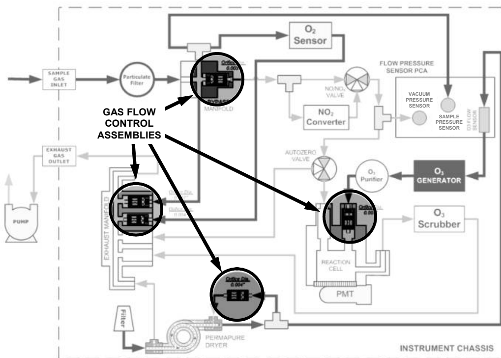
Figure 10-8: Location of Gas Flow Control Assemblies for M200EH with O 2 sensor Option 65
