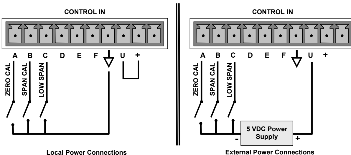
Figure 3-6: Control Input Connector
