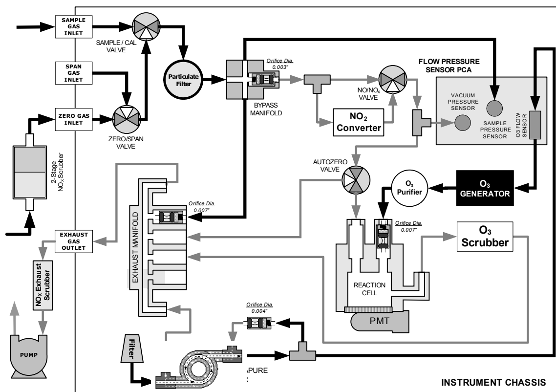
Figure 11-6: M200EH – Internal Gas Flow With OPT 50
