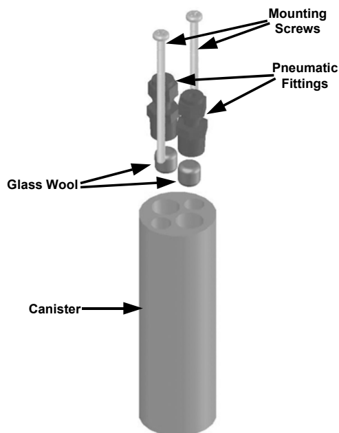
Figure 9-3: 04419 Ozone Filter Unit
