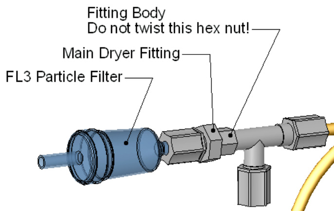
Figure 9-2: Particle Filter on O 3 Supply Air Dryer
