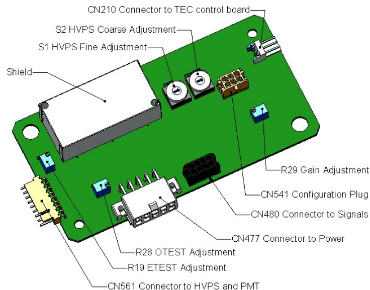
Figure 11-22: Pre-Amplifier Board Layout
