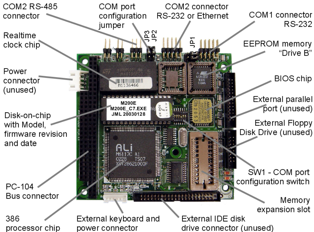
Figure 10-17: M200EH/EM CPU Board Annotated
