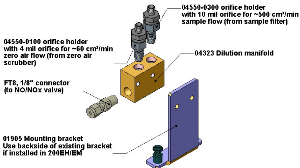
Figure 10-15: Dilution Manifold
