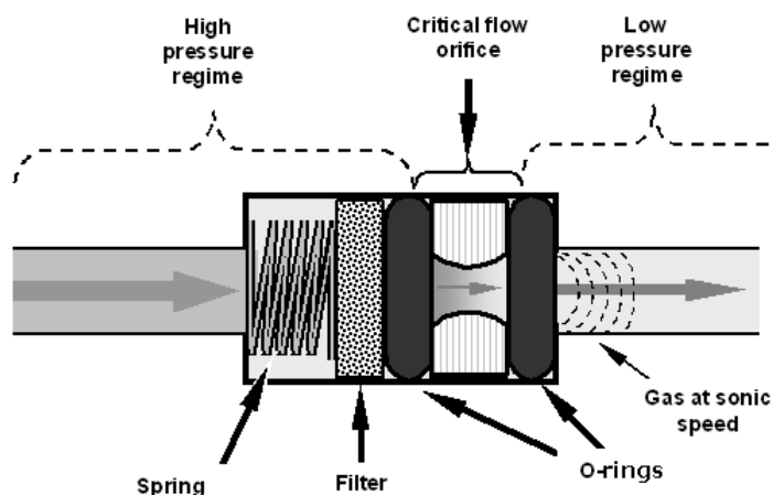
Figure 10-10: Flow Control Assembly & Critical Flow Orifice
