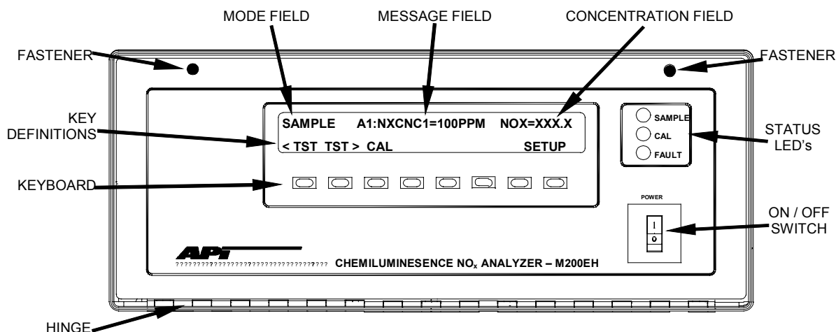
Figure 10-27: M200EH/EM Front Panel Layout
