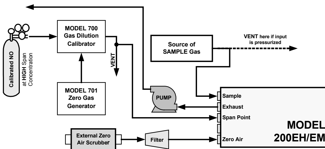
Figure 7-2: Pneumatic Connections—With Zero/Span Valve Option (50)
