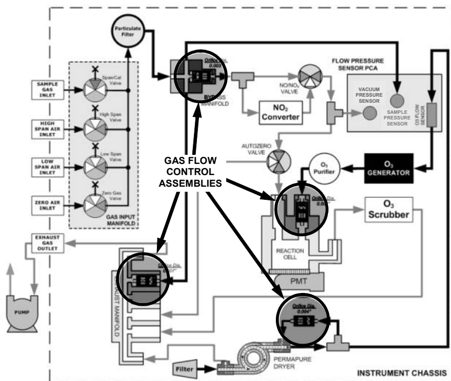
Figure 10-9: Location of Gas Flow Control Assemblies for M200EH with Second Span Point Option 52
