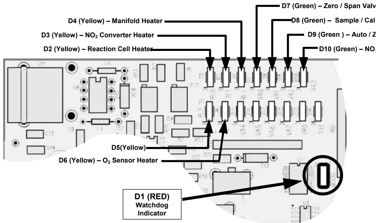
Figure 10-24: Status LED Locations – Relay PCA
