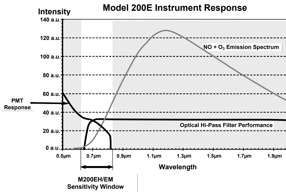
Figure 10-1: M200EH/EM Sensitivity Spectrum
