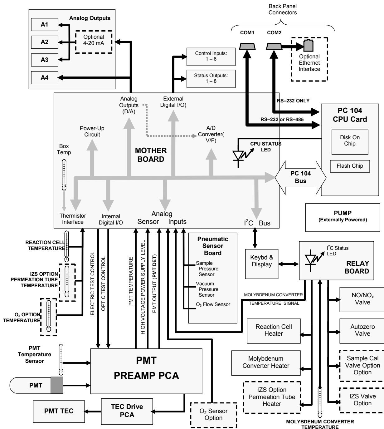
Figure 10-16: M200EH/EM Electronic Block Diagram
