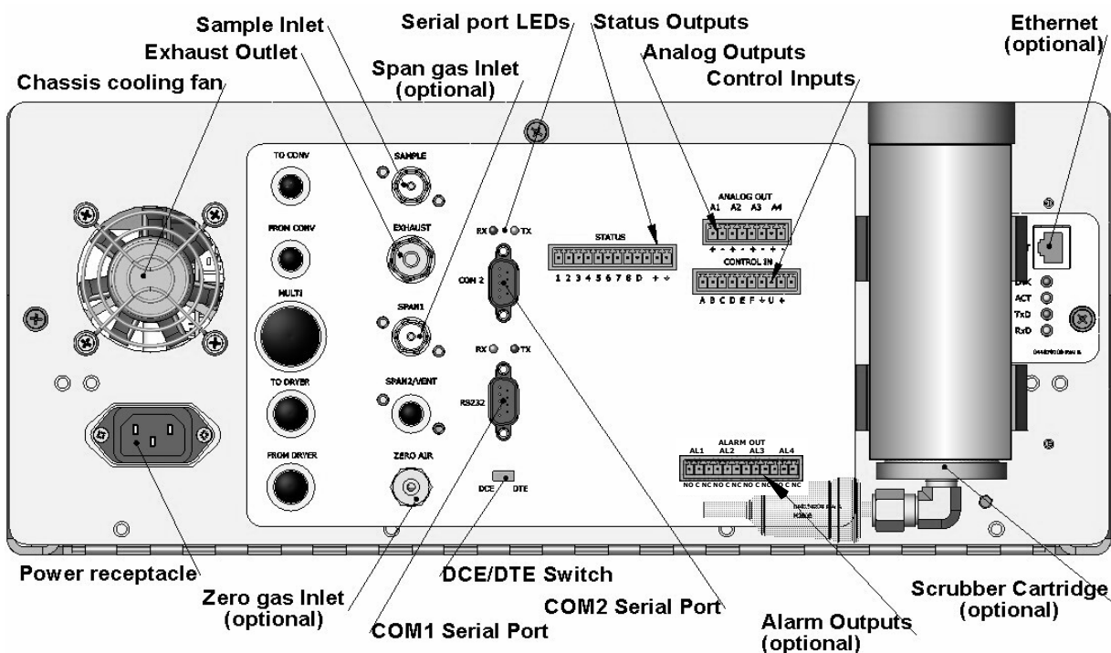
Figure 3-2: M200EH/EM Rear Panel Layout
