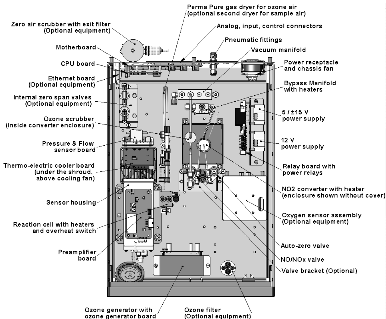
Figure 3-1: M200EH/EM Layout
