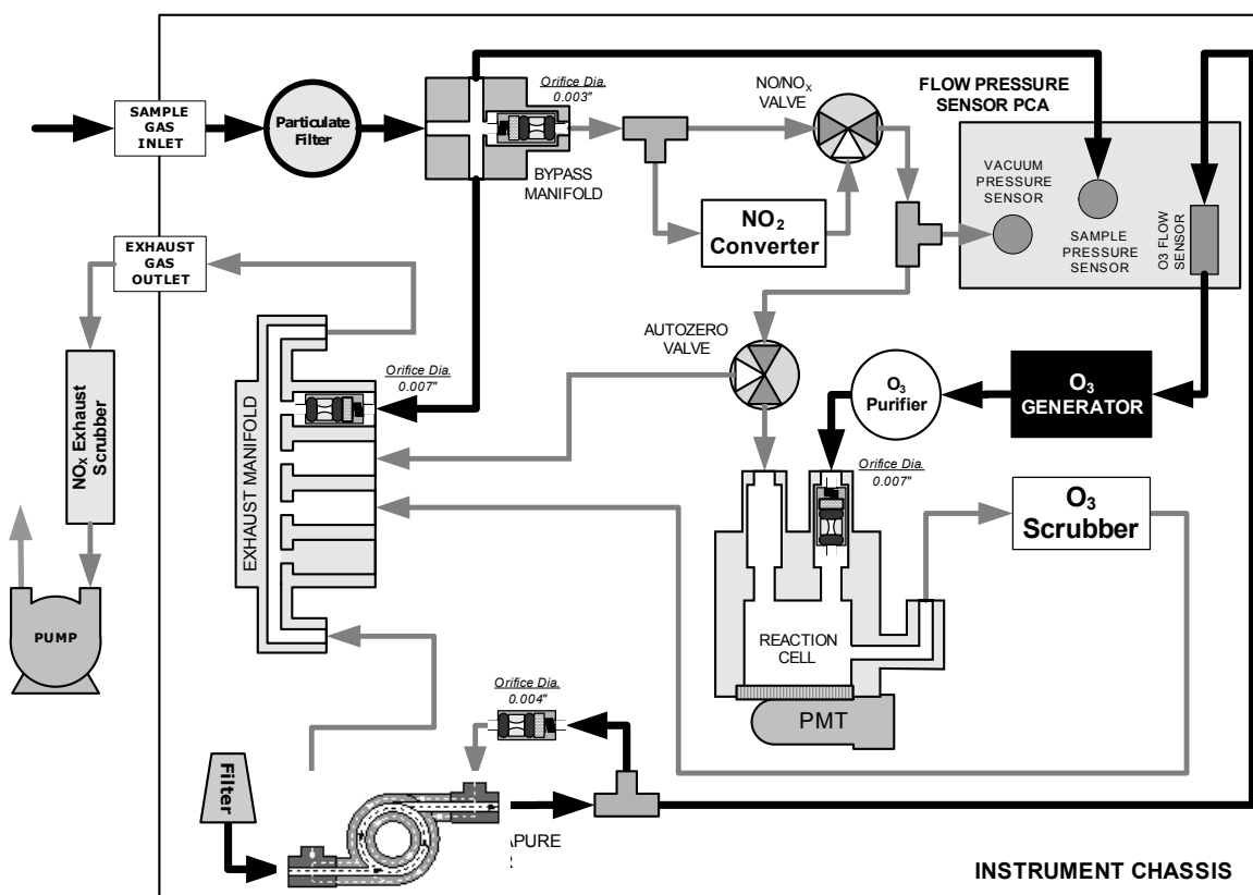
Figure 3-7: M200EH Internal Pneumatic Block Diagram - Standard Configuration
