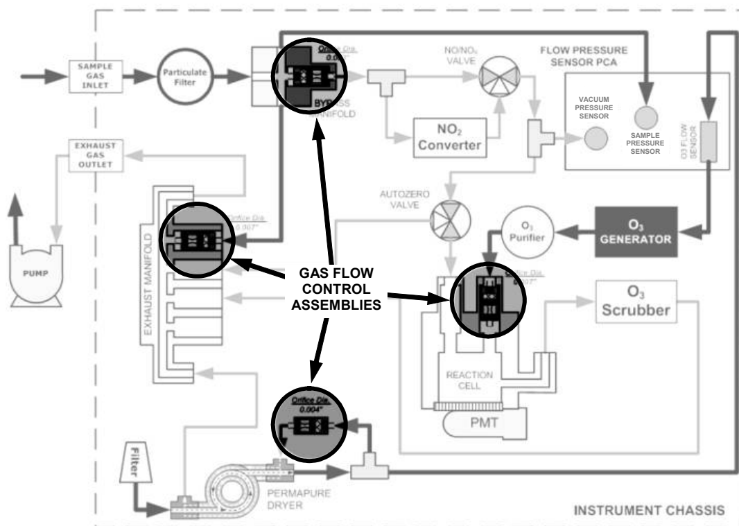
Figure 10-6: Location of Gas Flow Control Assemblies for M200EH
