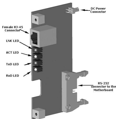
Figure 5-11: M200EH/EM Ethernet Card
