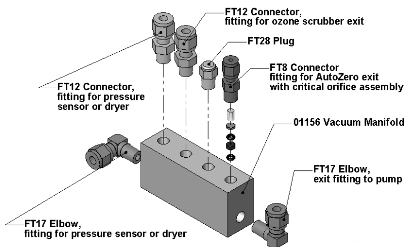
Figure 10-14: Vacuum Manifold
