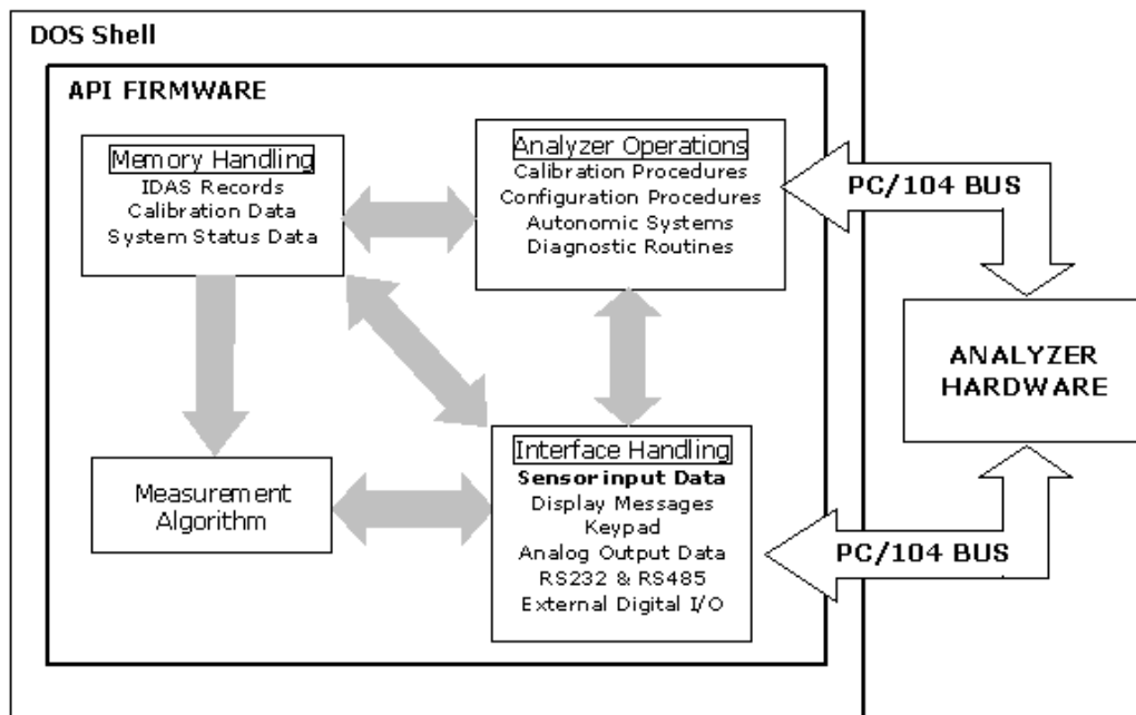
Figure 10-29: Schematic of Basic Software Operation
