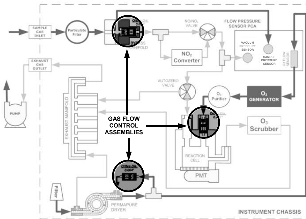
Figure 10-7: Location of Gas Flow Control Assemblies for M200EM
