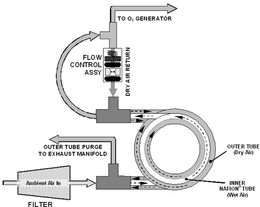
Figure 10-13: M200EH/EM Perma Pure® Dryer
