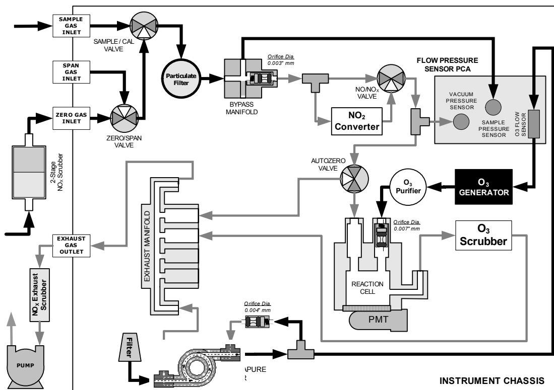
Figure 11-11: M200EM – Internal Gas Flow With OPT 50
