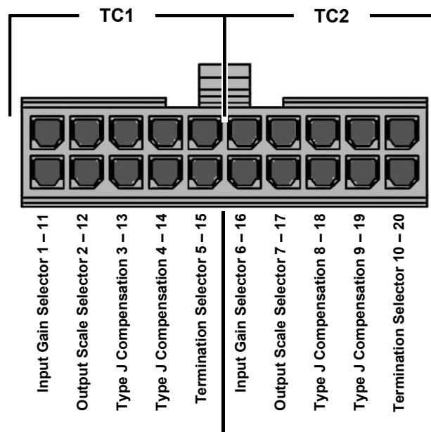
Figure 10-23: Thermocouple Configuration Jumper (JP5) Pin-Outs
