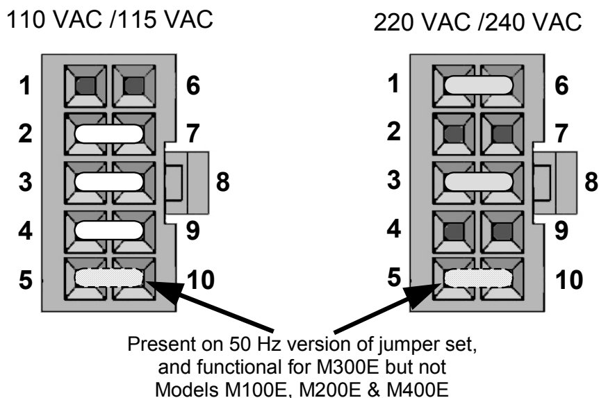
Figure 11-16: Pump AC Power Jumpers (JP7)
