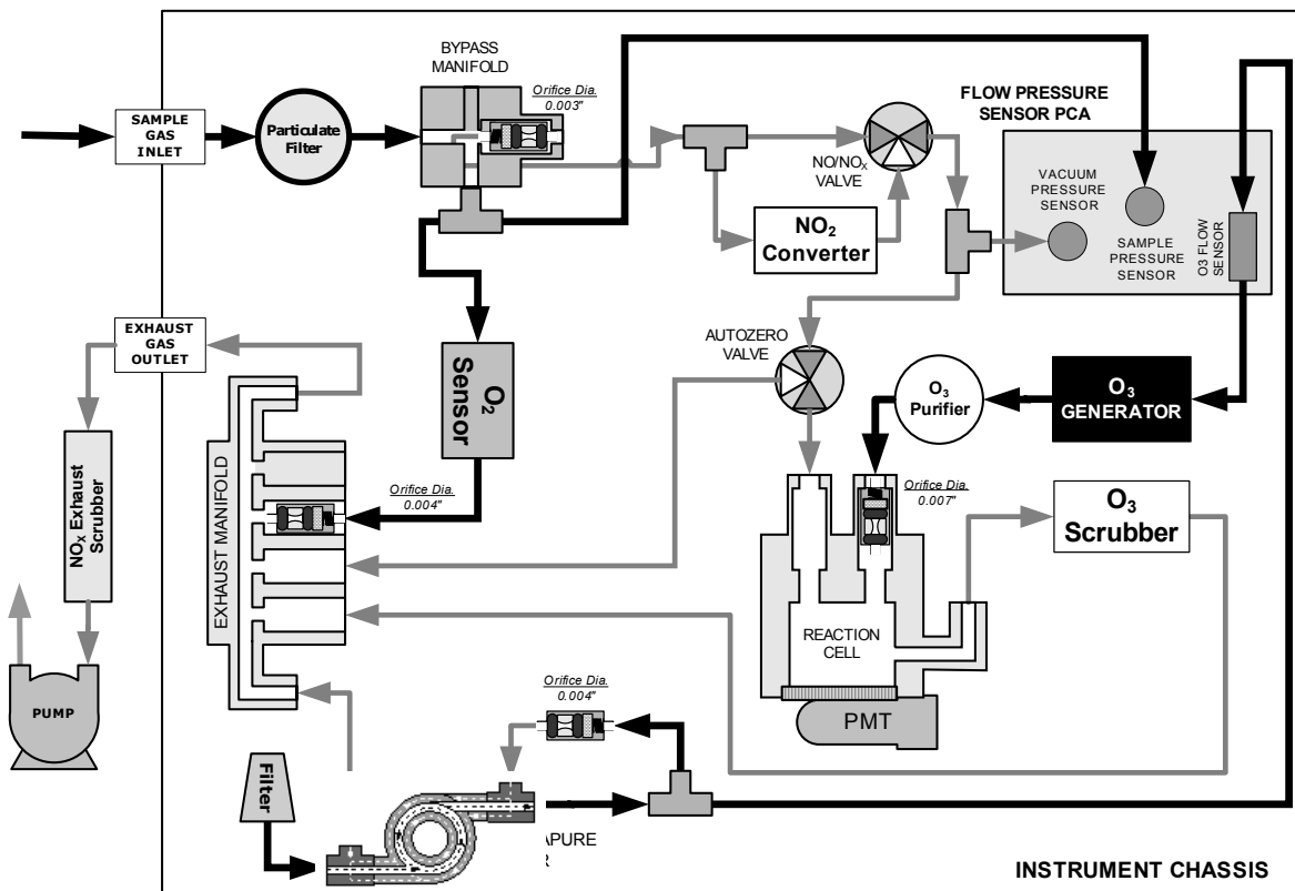
Figure 11-13: M200EM – Internal Gas Flow With OPT 65
