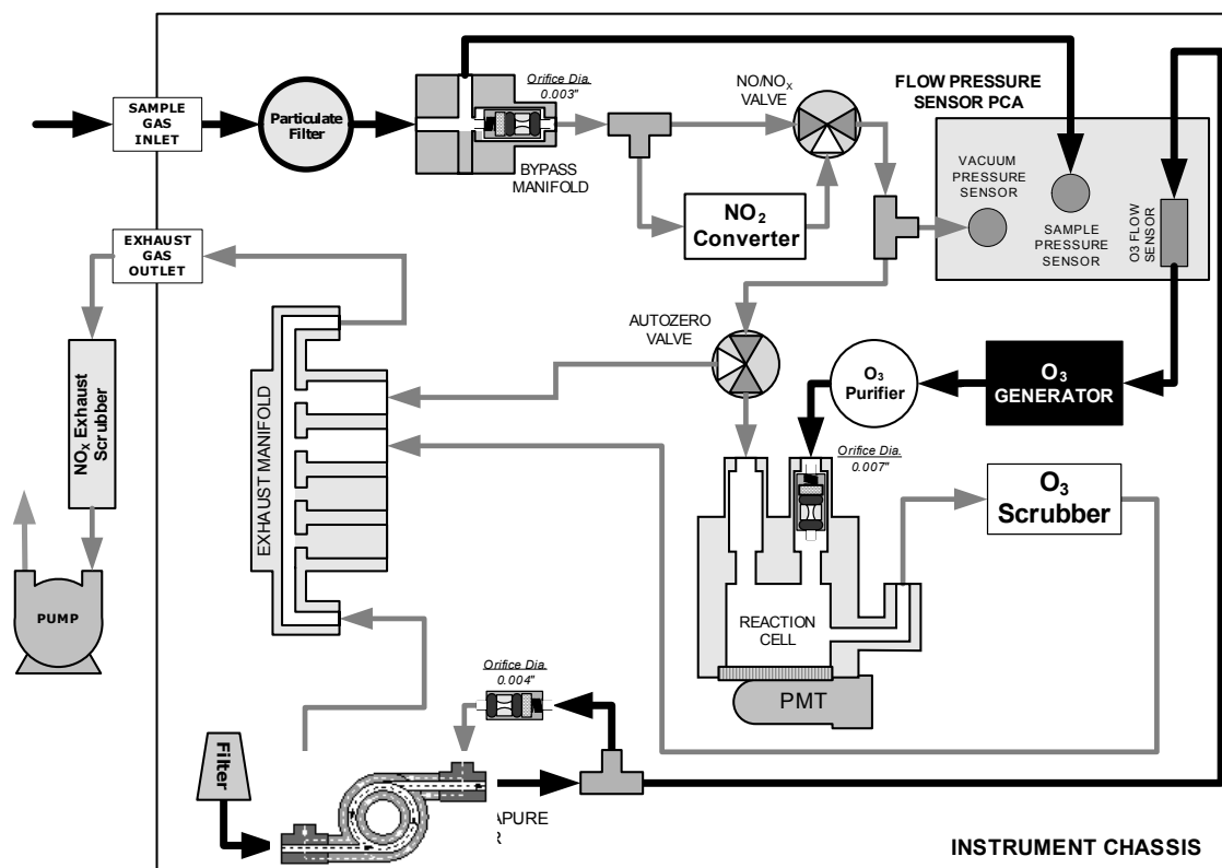
Figure 11-10: M200EM – Basic Internal Gas Flow
