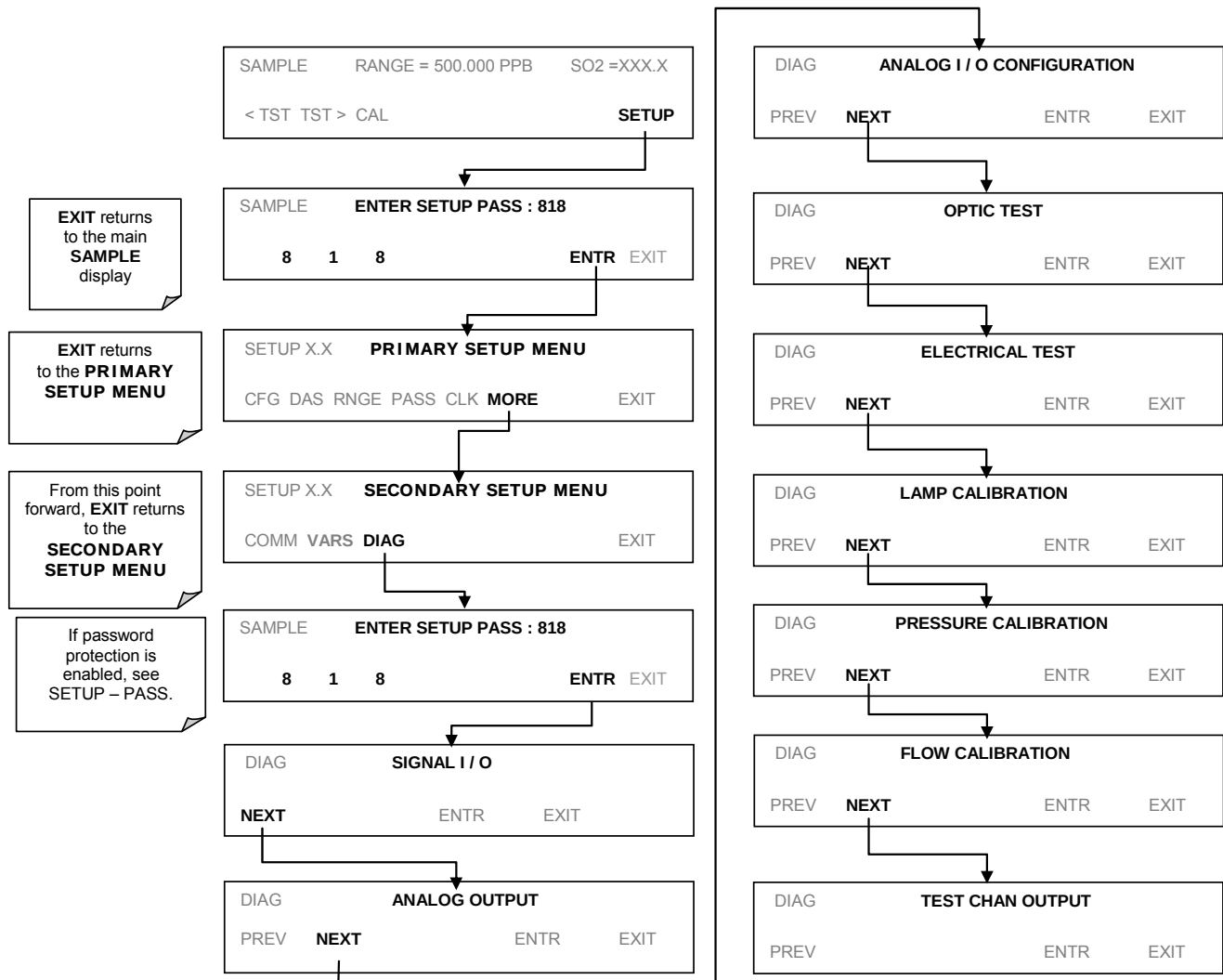
Figure 5-16: DIAG Menu
