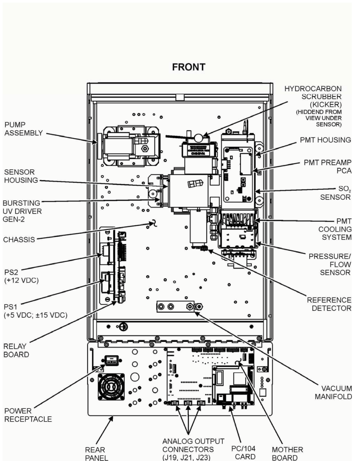
Figure 3-5: Internal Layout, Basic (no Valve or Second Gas Options)
