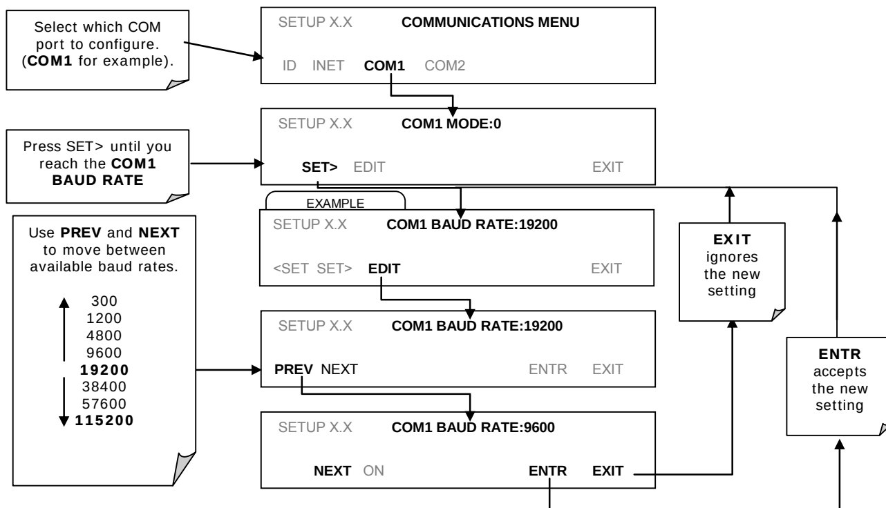
Figure 6-2: COMM – COMM Port Baud Rate
