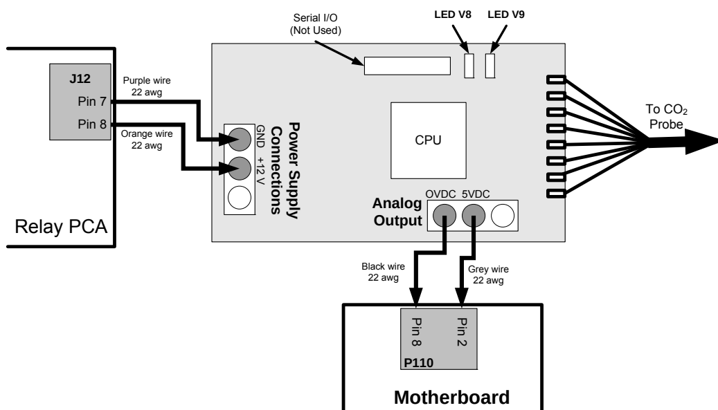
Figure 13-9: CO 2 Sensor Option PCA Layout and Electronic Connections
