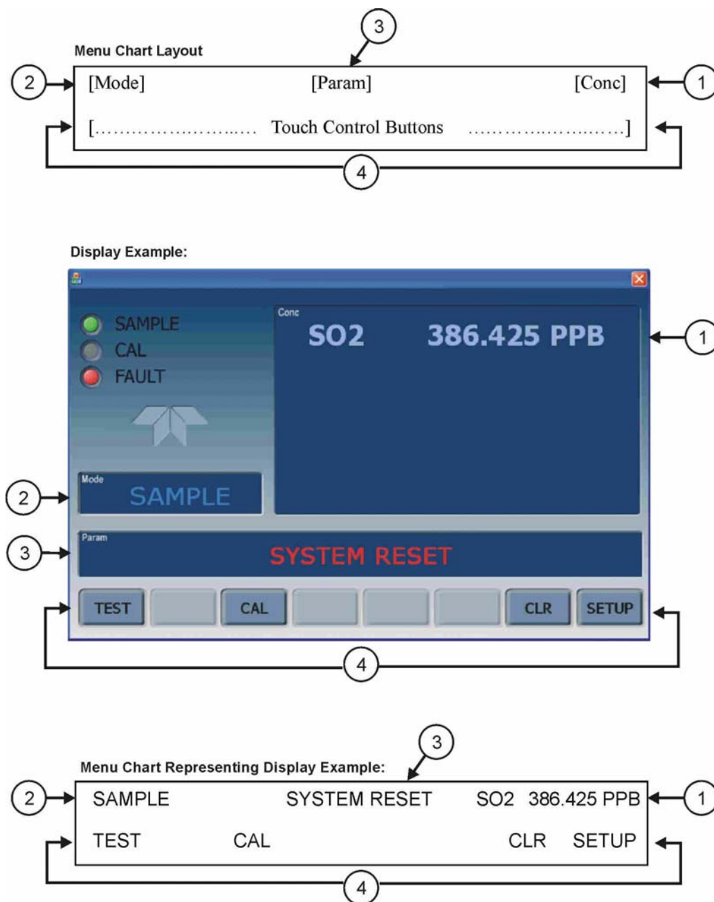
Figure 3-3: Display/Touch Control Screen Mapped to Menu Charts
