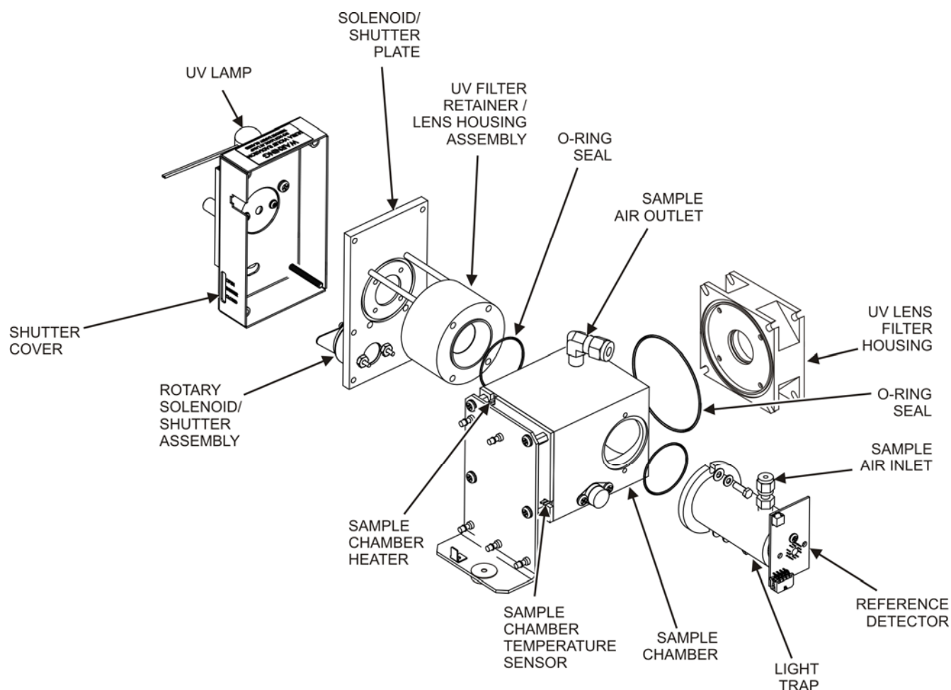
Figure 13-16: T100 Sample Chamber
