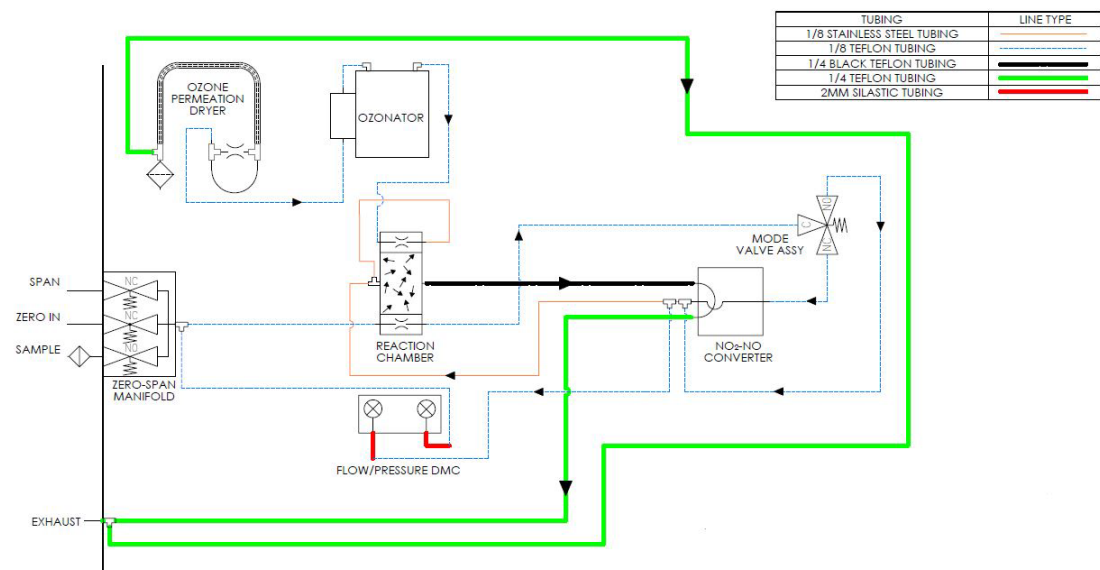
Figure 1–3. 42iQHL Flow Schematic with Zero Span
