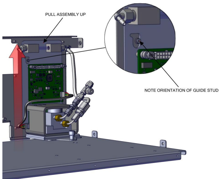
Figure 7–60. Oxygen Sensor Removal pt 3
