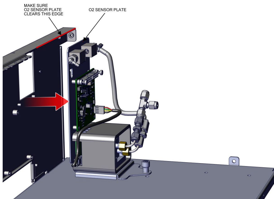
Figure 7–61. Oxygen Sensor Removal pt 4
