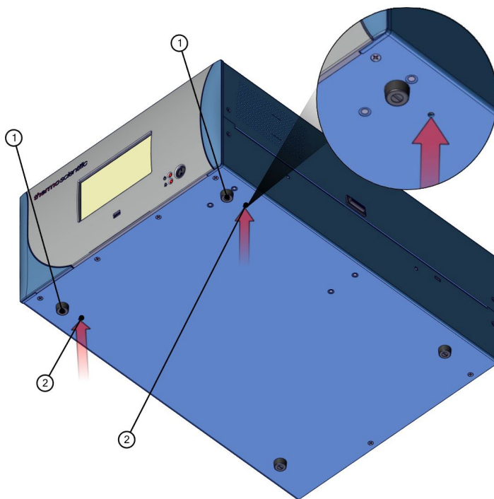
Figure 2–2. Installing Feet
