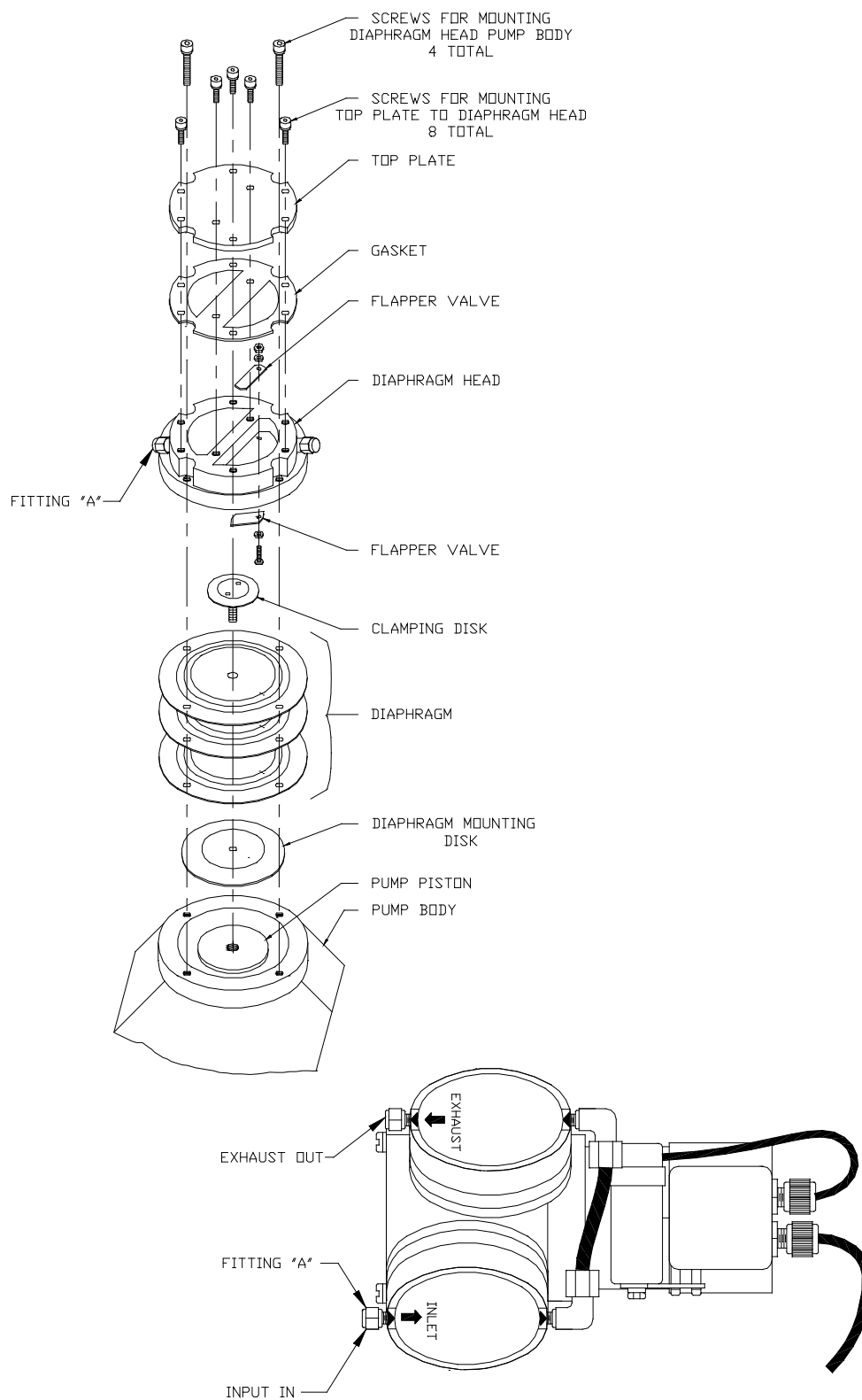
Figure 5-2. Pump Rebuilding
