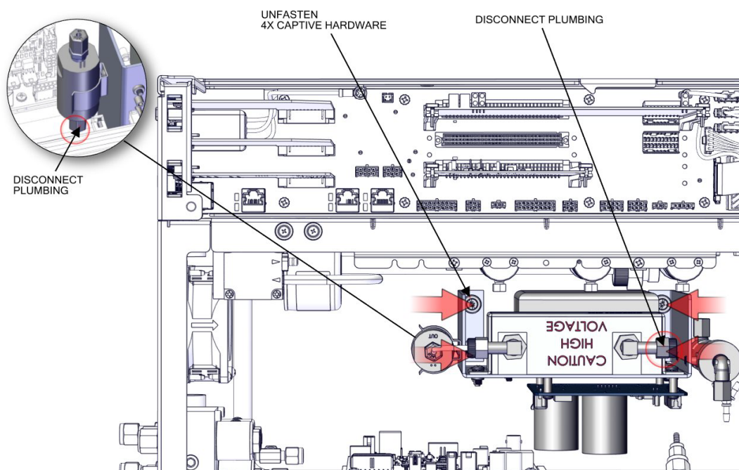
Figure 7-47. HVPS Remove
