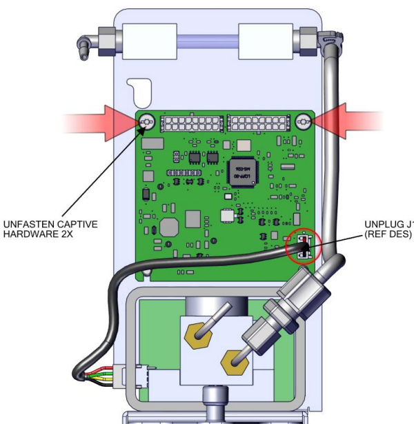
Figure 7–62. Replacing the Oxygen Sensor DMC Board
