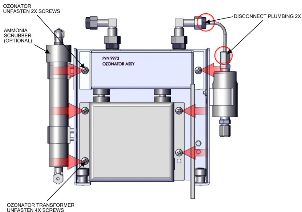
Figure 7–49. Replace Transformer
