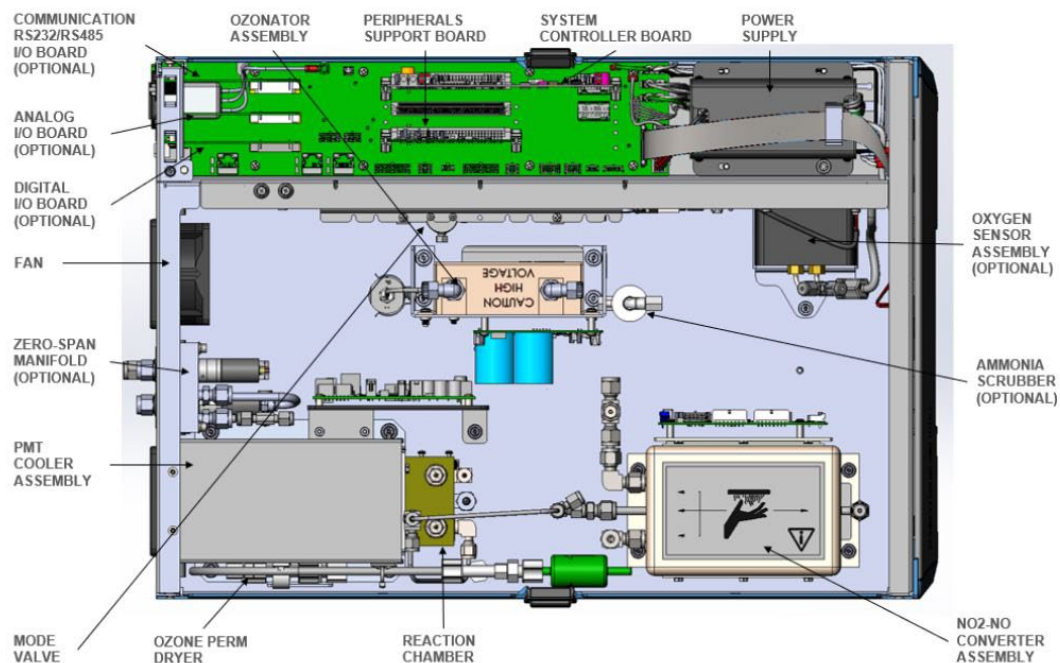
Figure 7-2. 42iQHL Component Layout Top View
