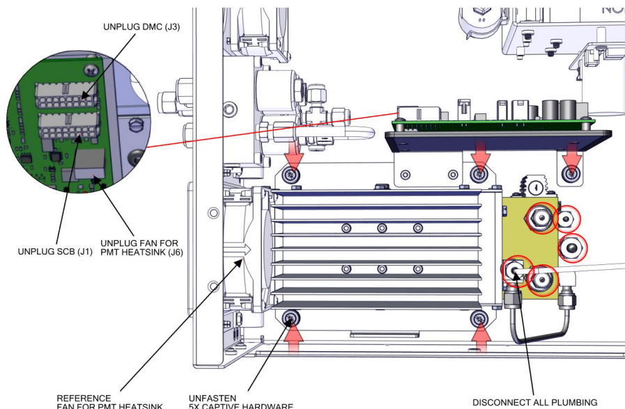
Figure 7–34. Remove PMT Cooler
