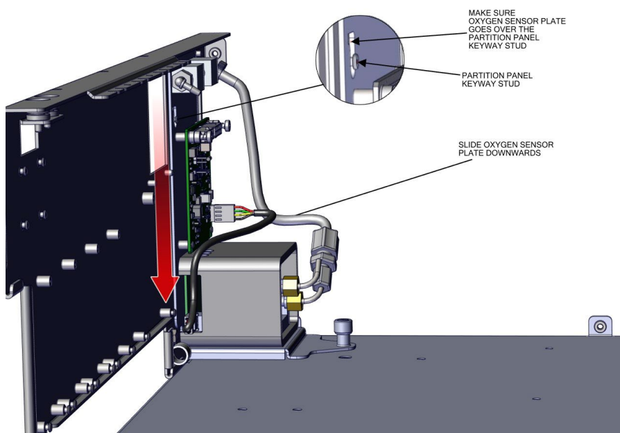
Figure 7-67. Installing the Oxygen Sensor DMC
