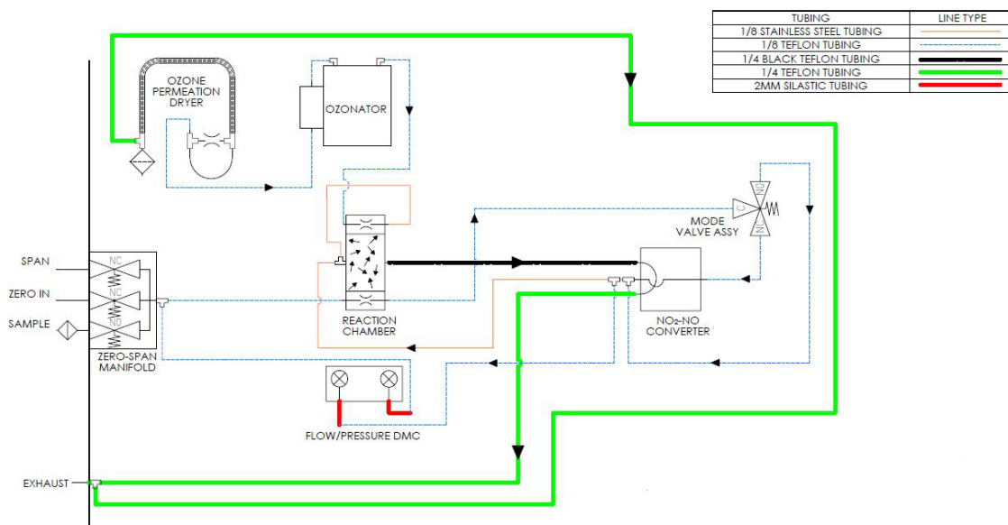
Figure 9–9. Flow Diagram, Zero/Span Option
