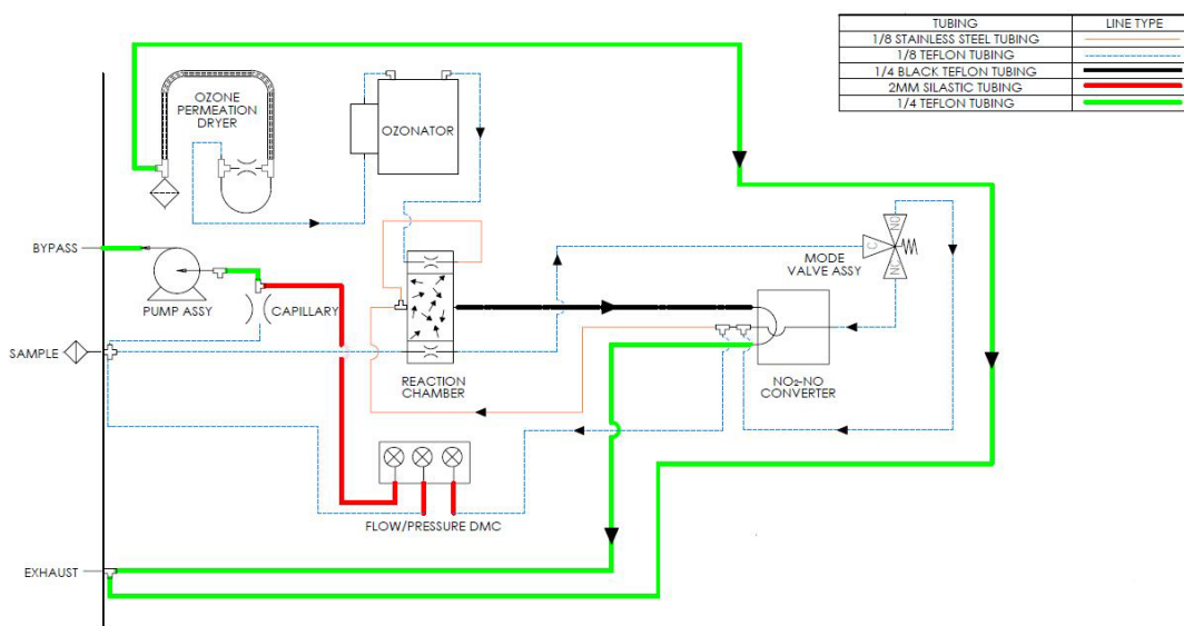
Figure 9–11. 42iQHL Flow Schematic with Bypass Flow Option
