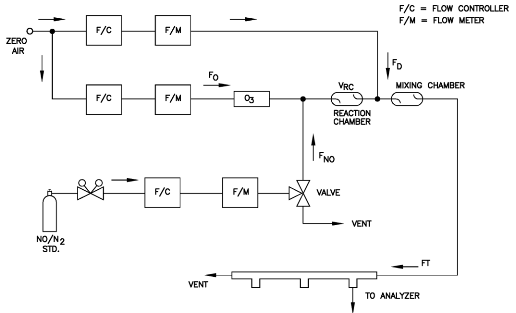
Figure 4–1. GPT System
