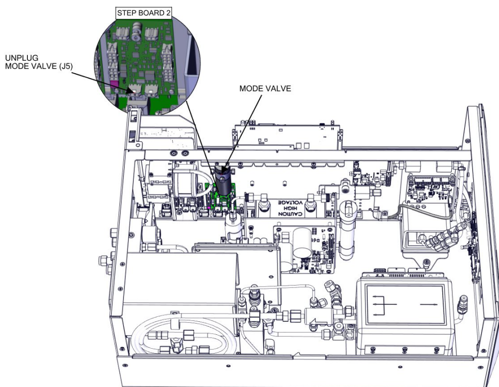
Figure 7–56. Mode Electrical Connection
