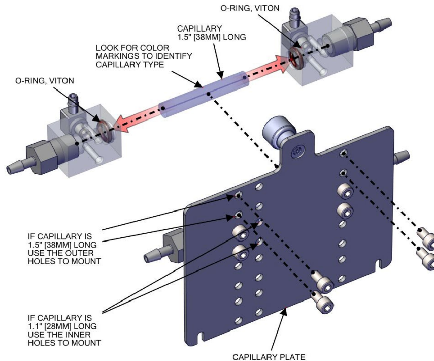
Figure 7-26. Capillary and O-Ring Replace
