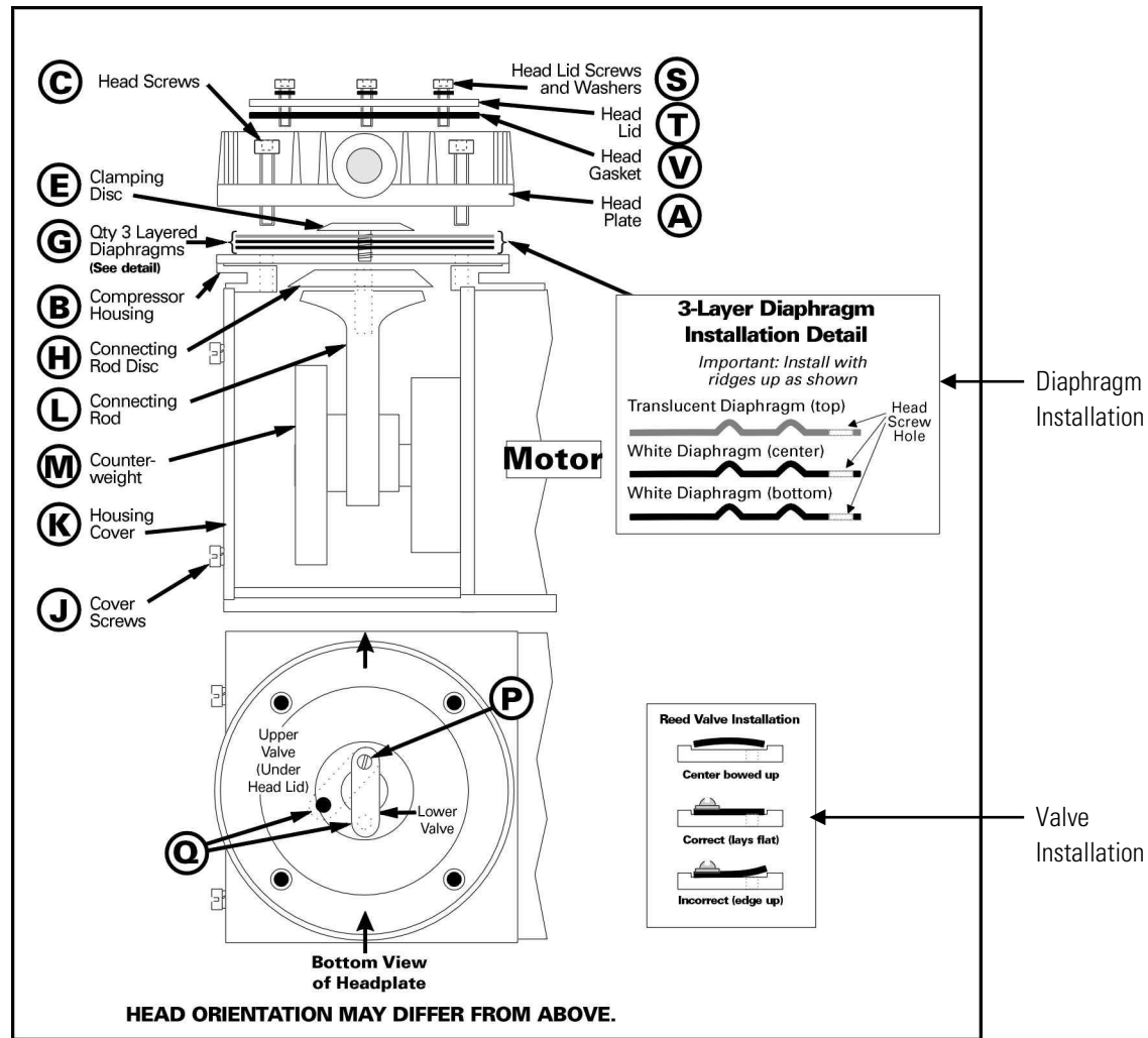
Figure 7-23. Vacuum Pump – Head Plate and Motor View
