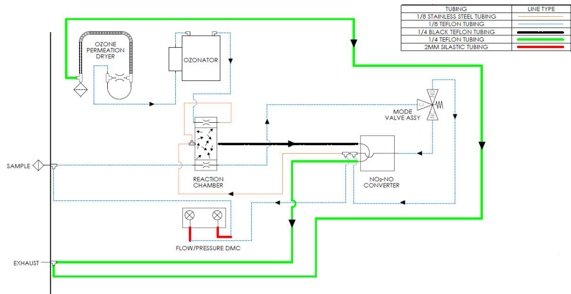
Figure 1–2. 42iQHL Flow Schematic
