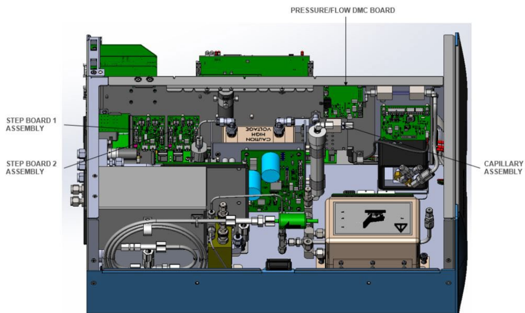
Figure 7-3. 42iQHL Component Layout Side View
