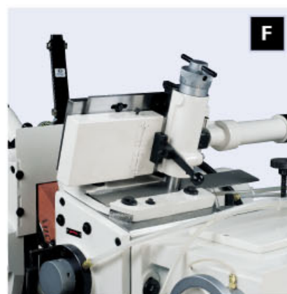
Dresser for Regulating wheel & Grinding Wheel (For I Axis)
