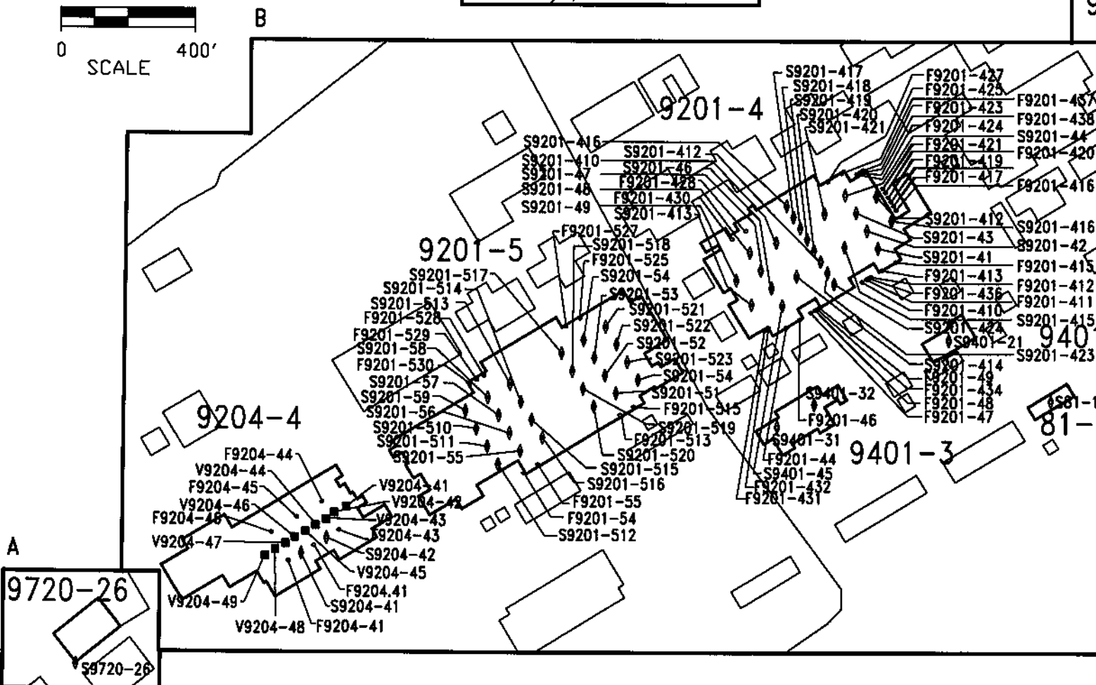
FIGURE 7-1 Y-12 PLANT AIRBORNE MERCURY RELEASE POINTS
