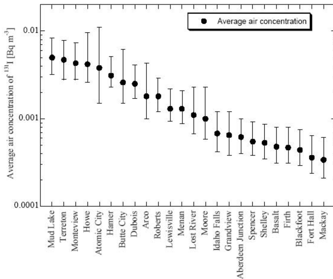
Figure 5.3 Estimated concentrations of iodine-131 in air averaged over the period of release (February 1957 – December 1959) at different offsite locations
