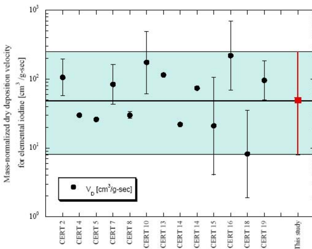
Figure A.1 The mass-normalized dry deposition velocity for elemental iodine as derived from the CERT studies performed on the Idaho National Engineering Laboratory site ( Bunch 1968 ), and the deposition velocity used in this study
