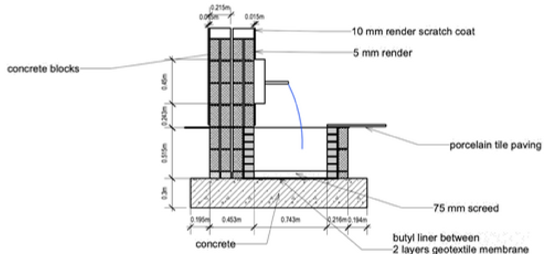
3 Section LM Wall Detail Scale 1:20
