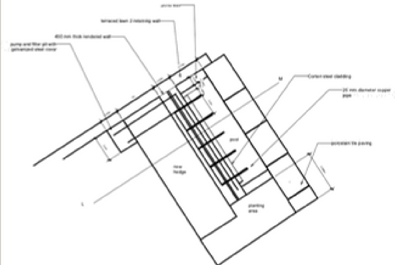
1 Water Feature Plan View Scale 1:20
