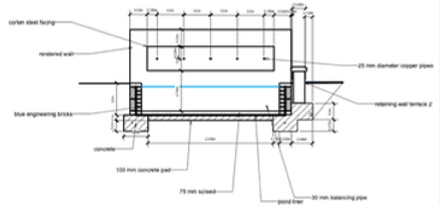
2 Water Feature Elevation Scale 1:20
