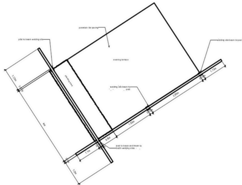
1 Evening Terrace Plan View Scale: 1:50
