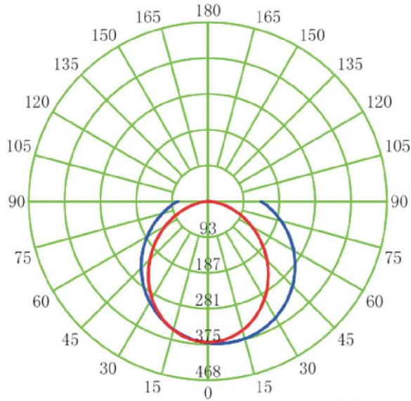
T8INT-2FTX-XX-YYXXX (X) LUMINOUS INTENSITY DISTRIBUTION DIAGRAM
