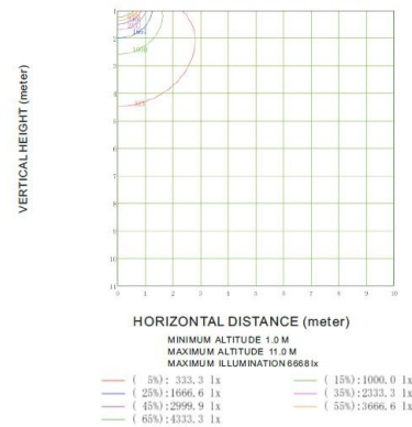
VERTICAL EQUILUMINOUS CURVE
