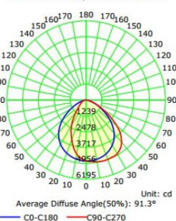
Luminous Intensity Distribution Curve
