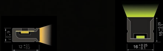
Conger Series Profile Cross Section
