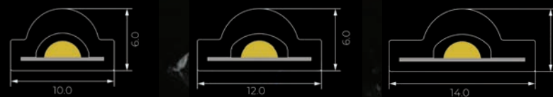
Hydra Series Profile Cross Section
