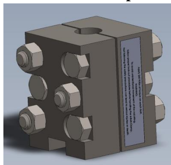
6-Bolt Clamp
