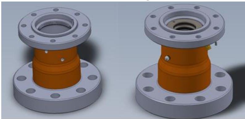
Seal Housing
