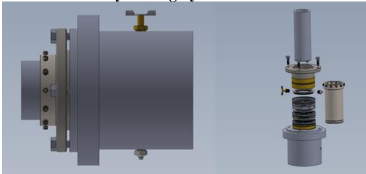
Assembly Sealing System 3000
