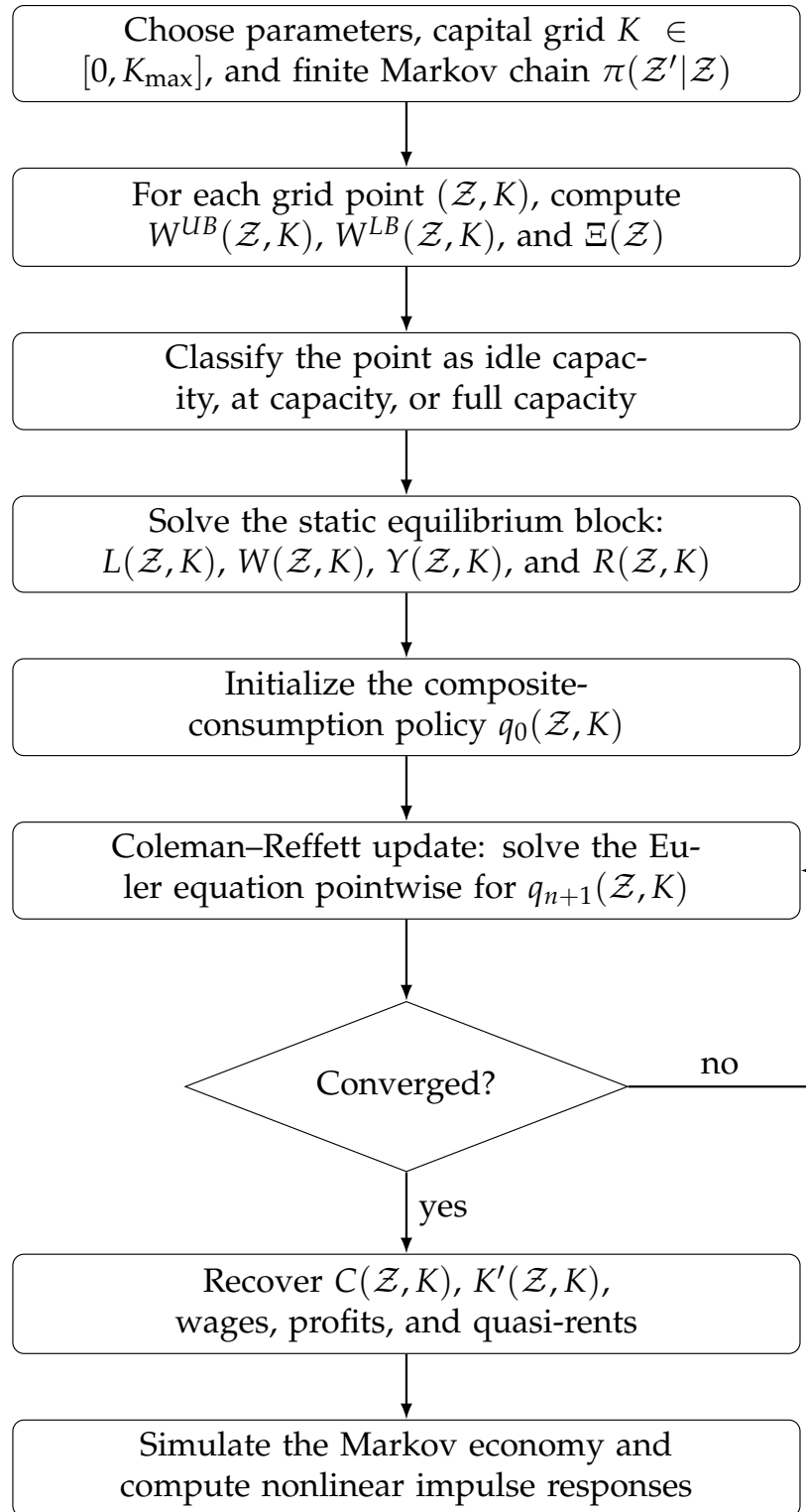
Figure 3: Time-Iteration Algorithm
